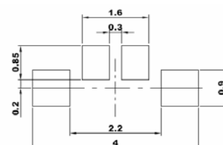
Recommended Soldering Pad Layout
