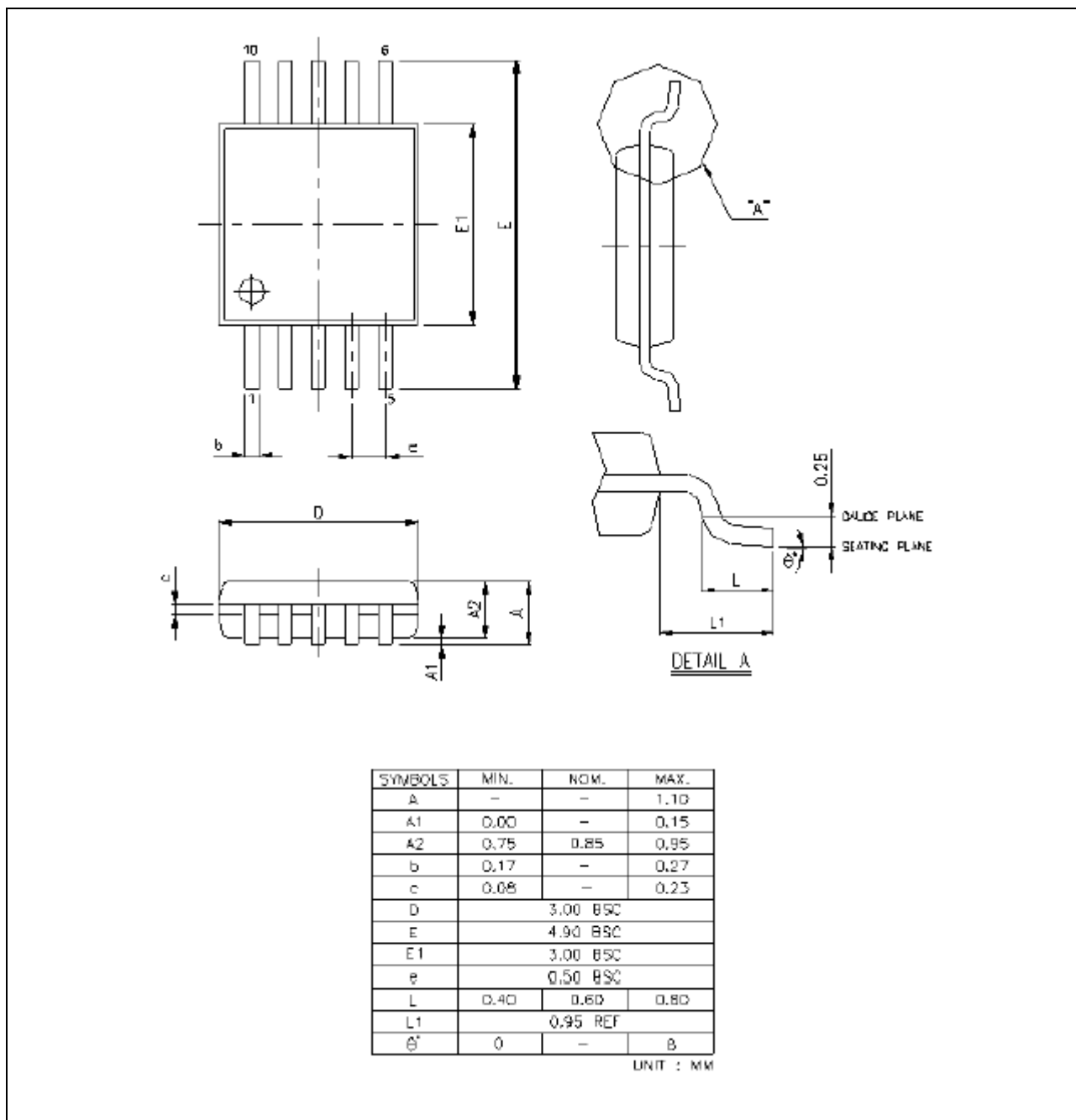
Figure 8.10-1 MSOP-10 Package Dimension
