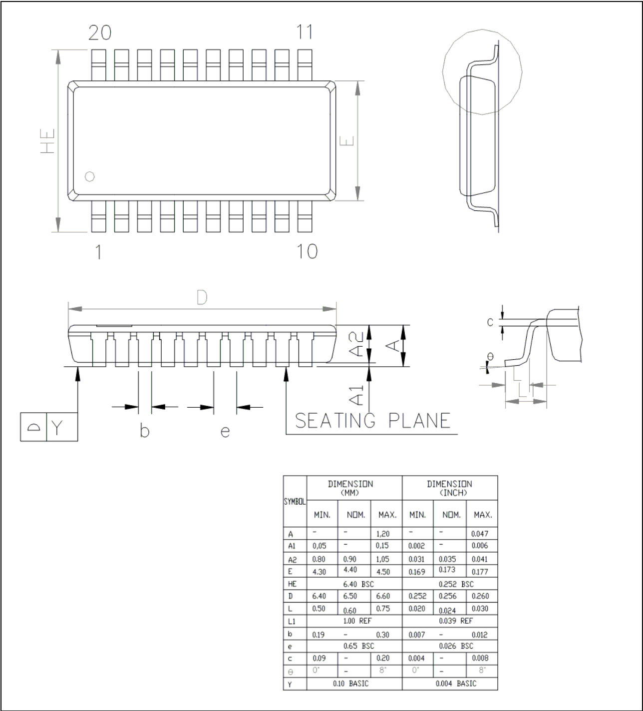
Figure 8.6-1 TSSOP-20 Package Dimension
