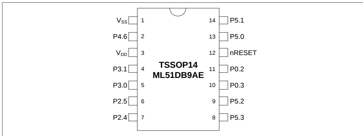
Figure 4.1-8 Pin Assignment of TSSOP-14 Package
