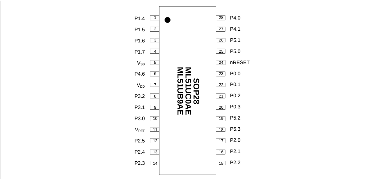
Figure 4.1-4 Pin Assignment of SOP-28 Package
