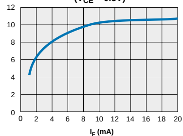
LDA100/LDA101 Typical Collector Current vs. Forward Current ( V_{CE} = 0.5V )
