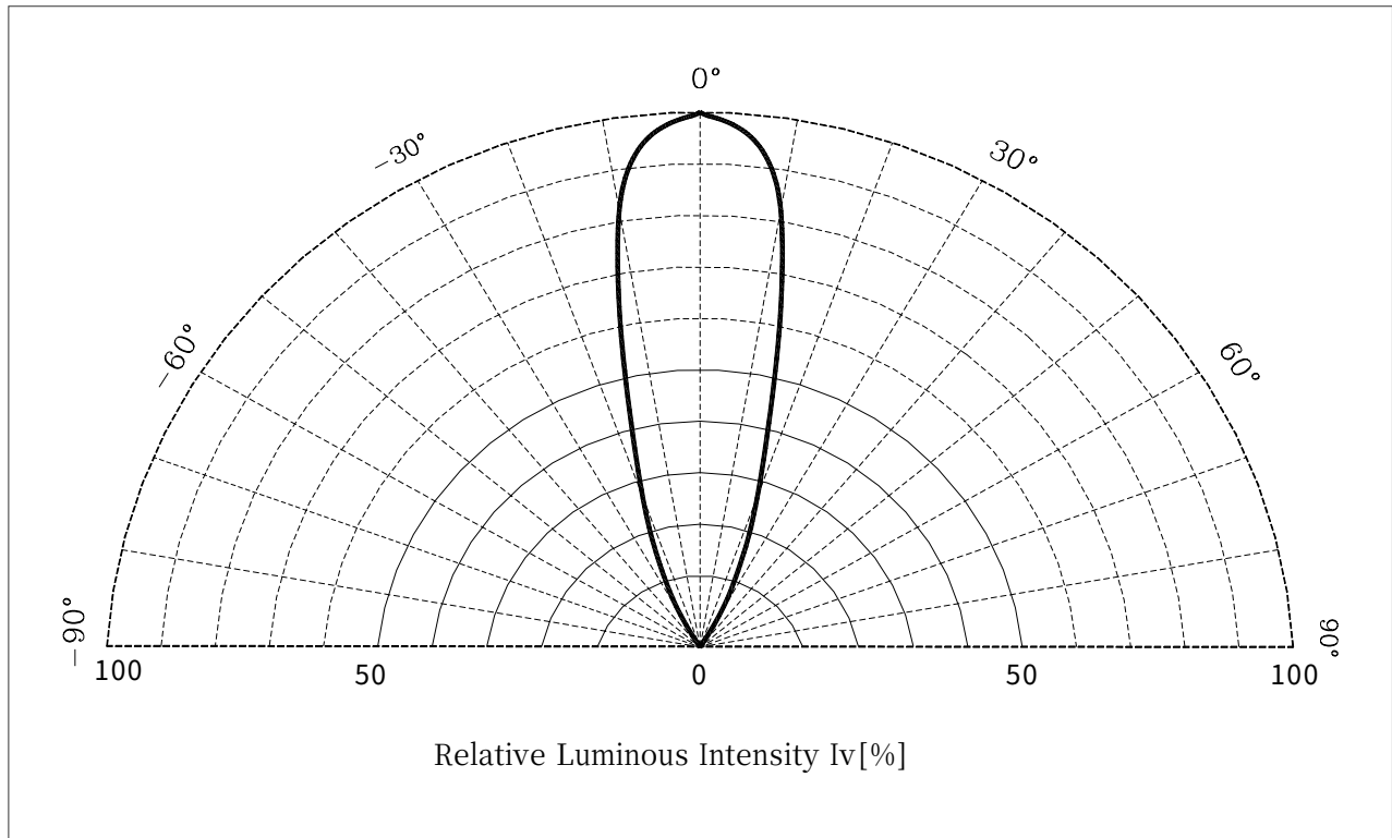
Fig. 5 Radiation Characteristics
