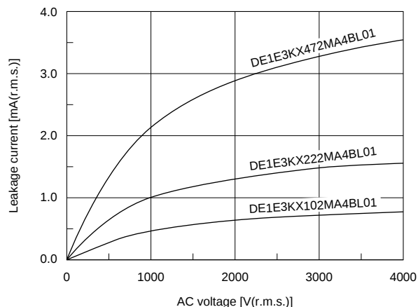
Type KX Small Size (E char.)
