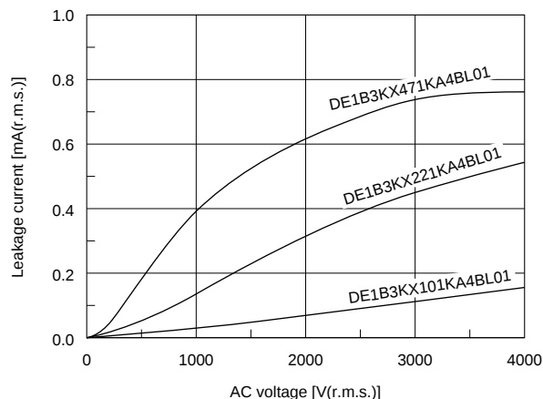
Type KX Small Size (B char.)
