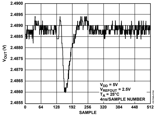
Figure 36. DAC-to-DAC Crosstalk
