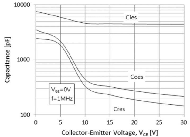
Fig.8 Typical Capacitance
