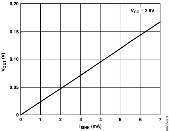
Figure 9. Voltage Output Low vs. I_{SINK}
