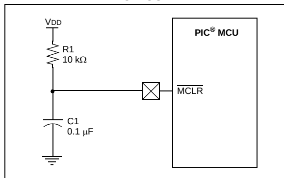
FIGURE 3-2: RECOMMENDED \overline{\text{MCLR}} CIRCUIT
