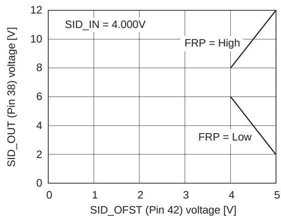
SID_OUT voltage vs. SID_OFST voltage (2)
