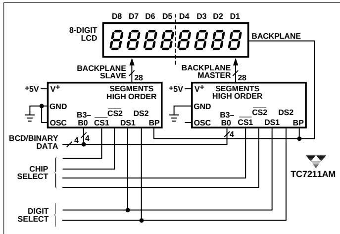
Figure 3. TC7211AM Driving an 8-Digit LCD Display in Master/Slave Configuration
