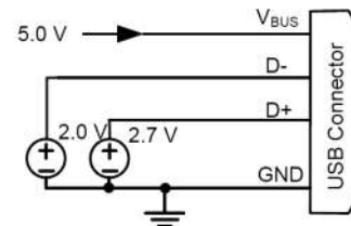
Fig 3. Divider 2 DCP
