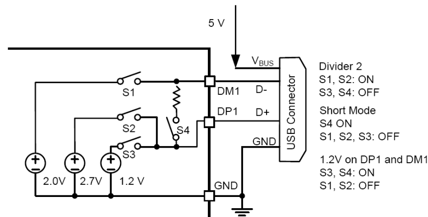
Fig 5. DCP Auto-Detect Functional Diagram
