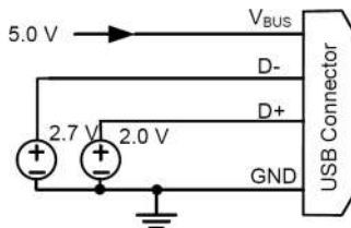
Fig 2. Divider 1 DCP
