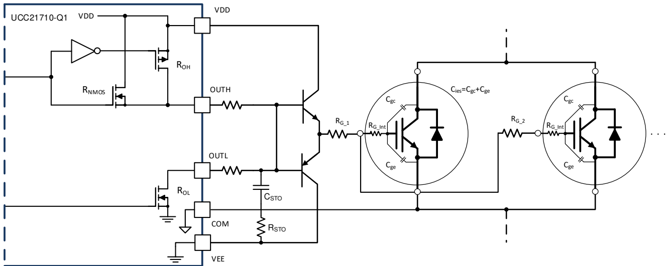
Figure 9-16. Current Buffer for Increased Drive Strength
