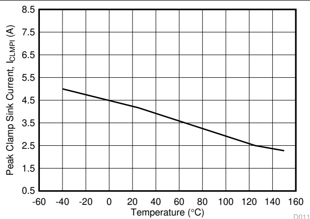
Figure 6-22. I CLMPI Miller Clamp Sink Current vs. Temperature
