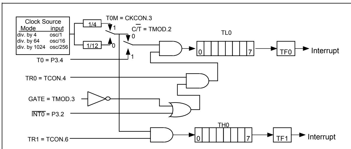
Figure 13: Timer/Counter 0 Mode 3
