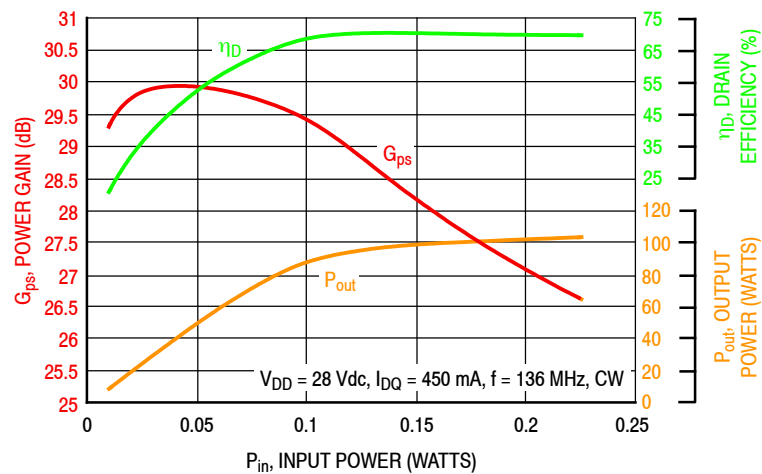
Figure 15. Power Gain, Output Power and Drain Efficiency versus Input Power
