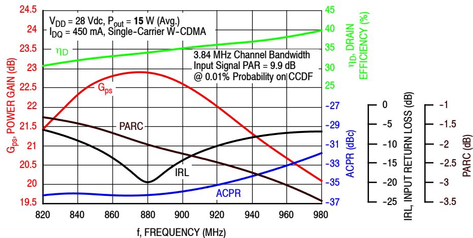
Figure 6. Single-Carrier Output Peak-to-Average Ratio Compression (PARC) Broadband Performance @ P_{out} = 15 Watts Avg.
