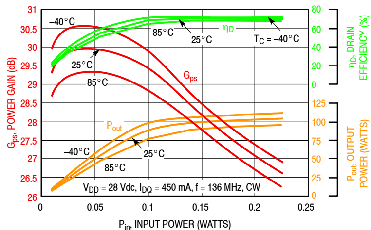
Figure 16. Power Gain, Output Power and Drain Efficiency versus Input Power over Temperature
