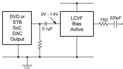
Figure 3. AC-Coupled Input and Output
