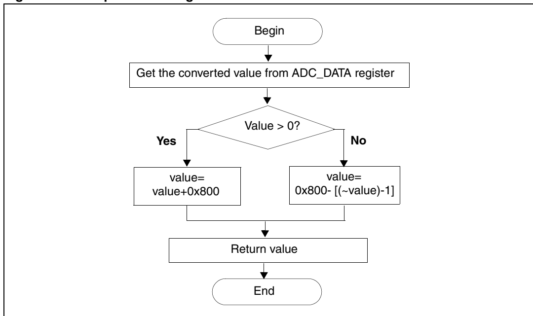
Figure 7. Compute the unsigned value of a converted value
