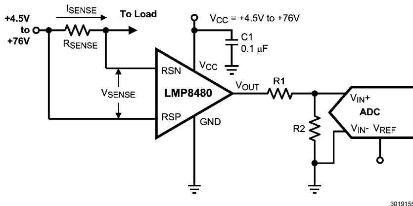
FIGURE 11. Typical Application with Resistive Divider
