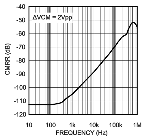
AC Common-Mode Rejection Ratio vs. Frequency
