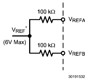
FIGURE 7. V_{REF} Input Resistor Network
