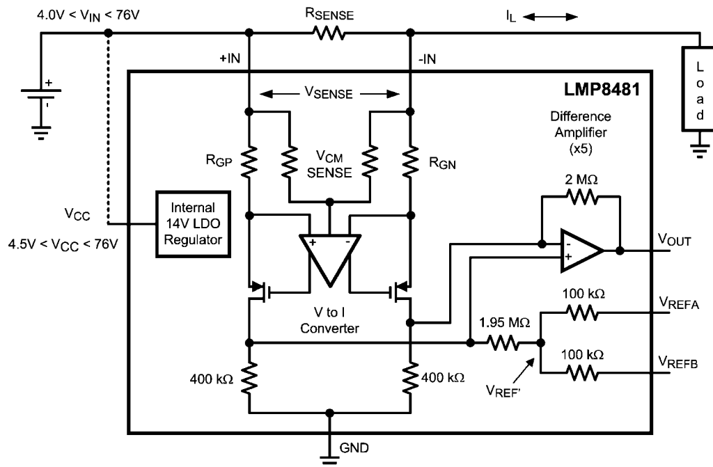
LMP8481 Block Diagram
