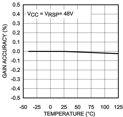
Typical Gain Accuracy vs. Temperature
