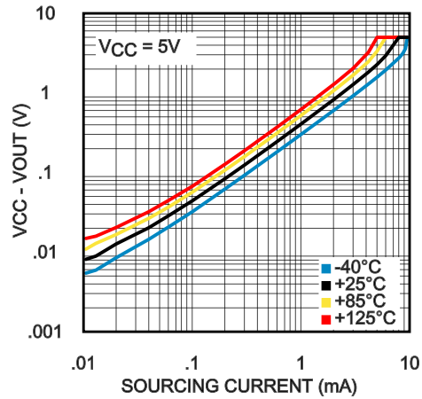
Saturated Output Sourcing Current at 4.5V
