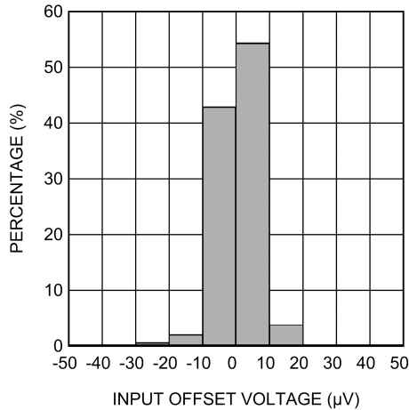
Offset Voltage Histogram
