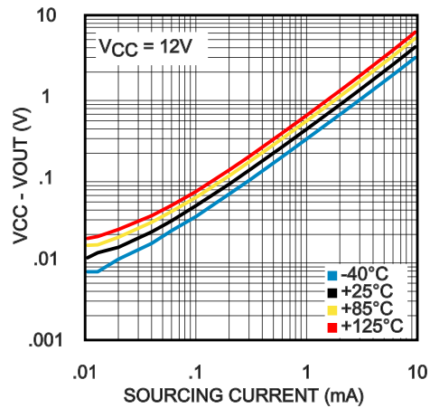
Saturated Output Sourcing Current at 12V
