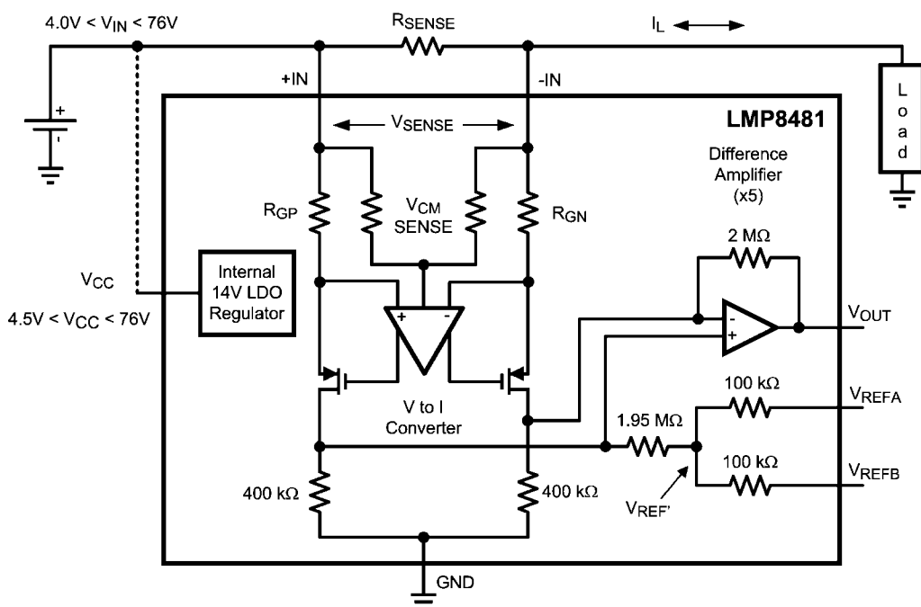
FIGURE 1. LMP8481 Functional Diagram
