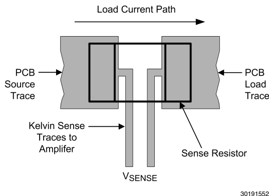
FIGURE 12. "Kelvin" or "4-wire" Connection to the Sense Resistor
