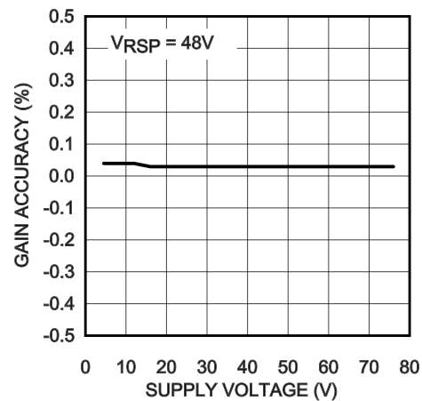
Typical Gain Accuracy vs. Supply Voltage
