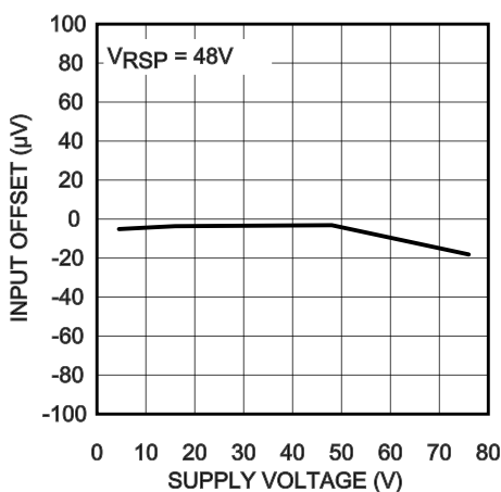
Typical Offset Voltage vs. Supply Voltage
