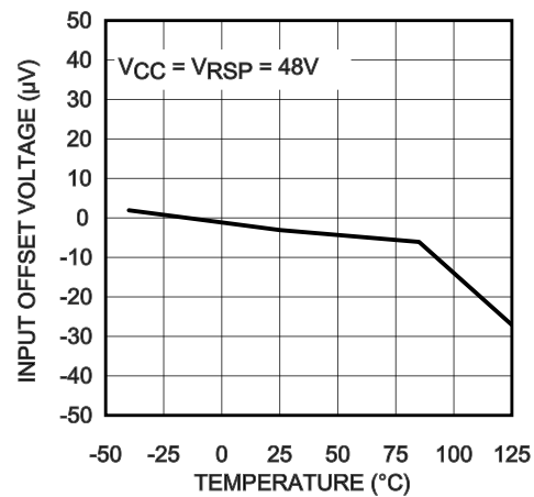
Typical Offset Voltage vs. Temperature
