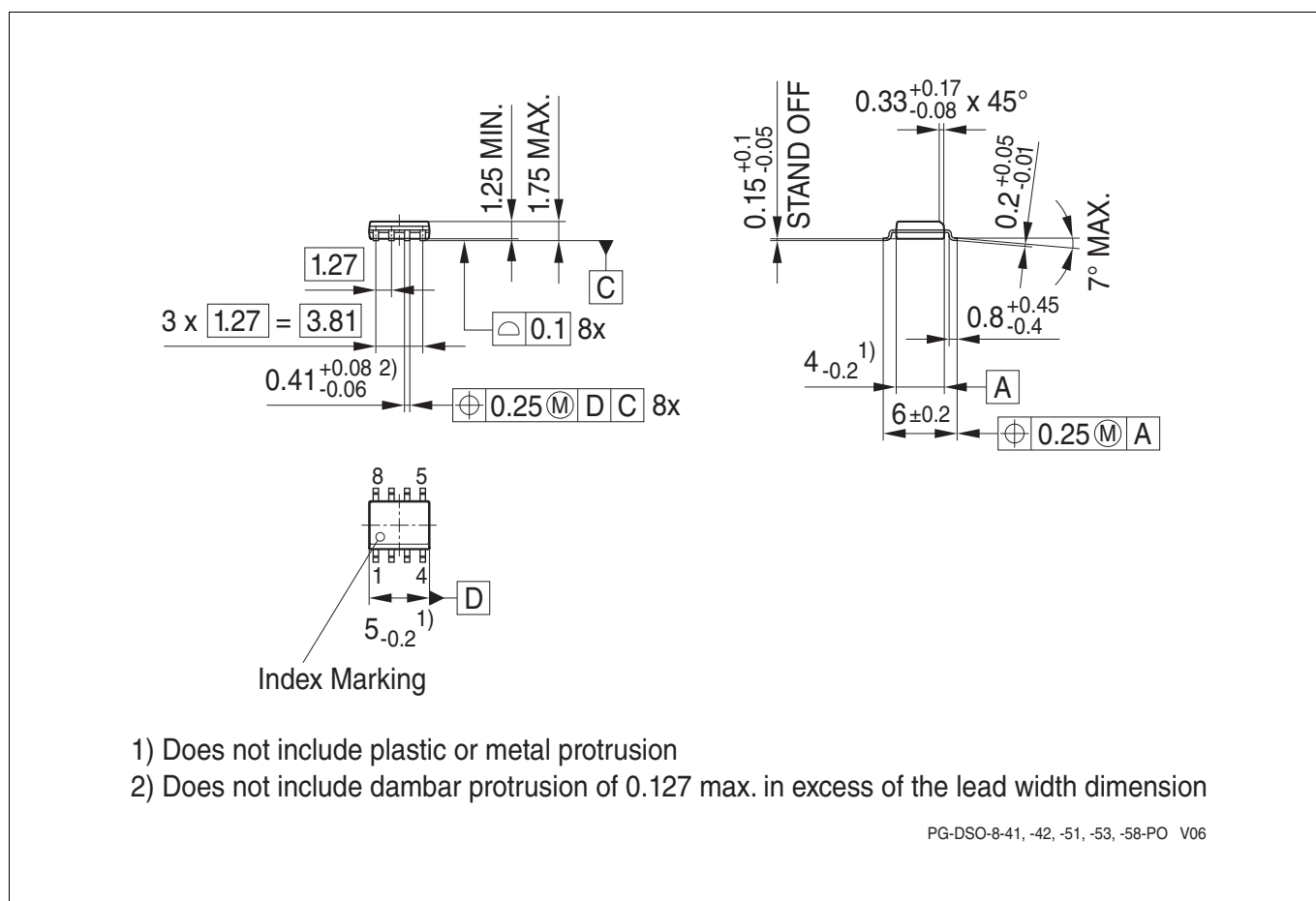
Figure 28 PG-DSO-8 outline 1)
