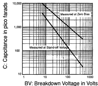
FIGURE 4 Typical Capacitance vs. Breakdown Voltage
