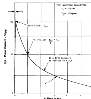
FIGURE 2 Pulse Wave Form
