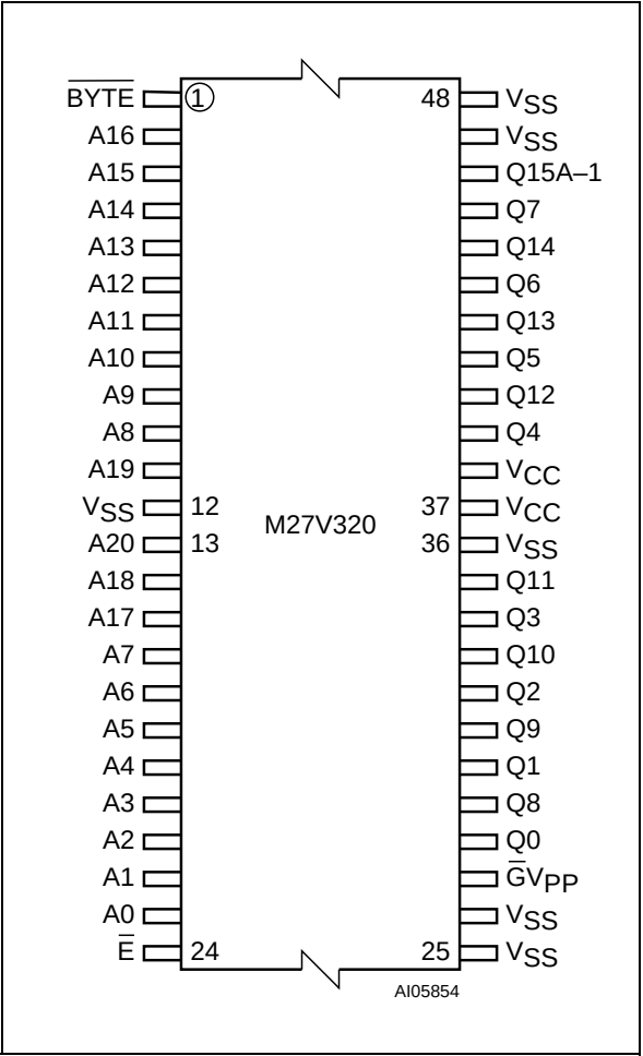
Figure 3. TSOP Connections
