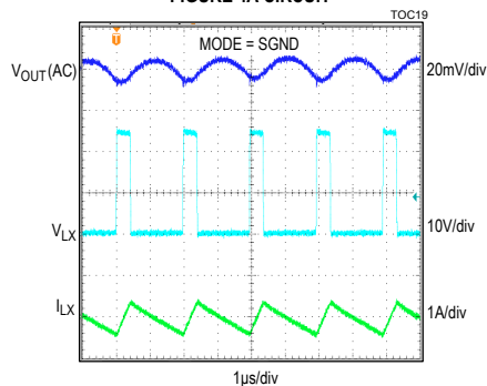
STEADY-STATE SWITCHING WAVEFORMS 5V OUTPUT, PWM MODE, NO LOAD, FIGURE 4A CIRCUIT
