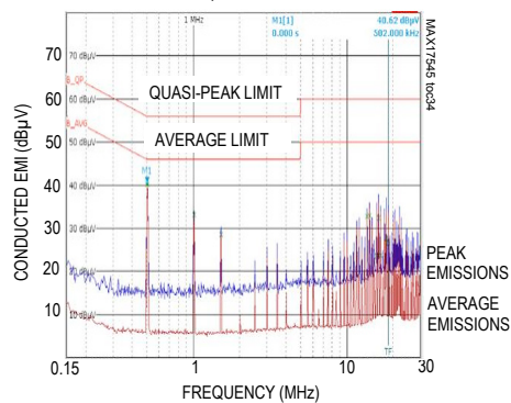
MAX17545 5V OUTPUT, 1.7A LOAD CURRENT, FIGURE 4A CIRCUIT, CONDUCTED EMI CURVE
