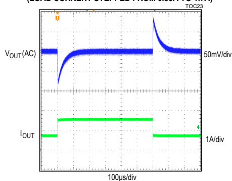
3.3V OUTPUT, PWM MODE, FIGURE 4B CIRCUIT (LOAD CURRENT STEPPED FROM 0.85A TO 1.7A)
