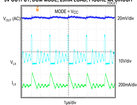
STEADY-STATE SWITCHING WAVEFORMS, 5V OUTPUT, DCM MODE, 25mA LOAD, FIGURE 4A CIRCUIT
