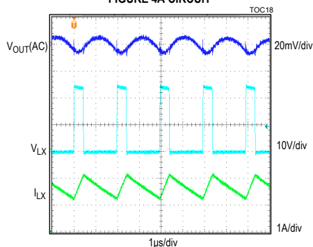
STEADY-STATE SWITCHING WAVEFORMS 5V OUTPUT, 1.7A LOAD CURRENT, FIGURE 4A CIRCUIT
