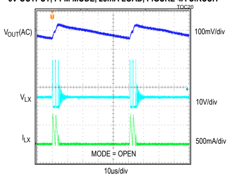
STEADY-STATE SWITCHING WAVEFORMS, 5V OUTPUT, PFM MODE, 25mA LOAD, FIGURE 4A CIRCUIT
