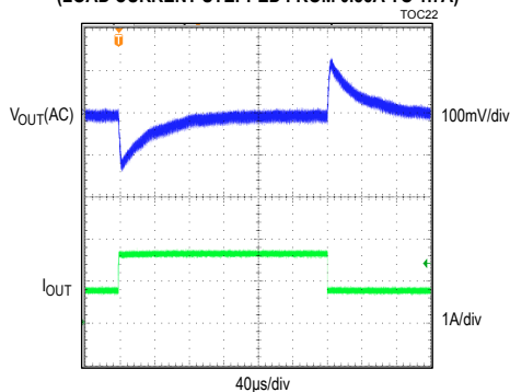
5V OUTPUT, PWM MODE, FIGURE 4A CIRCUIT (LOAD CURRENT STEPPED FROM 0.85A TO 1.7A)
