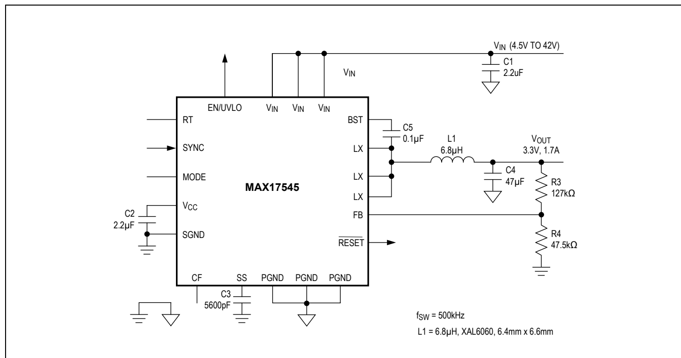
Typical Application Circuits (continued)
