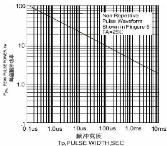
FIG. 5–PULSE RATING CURVE
