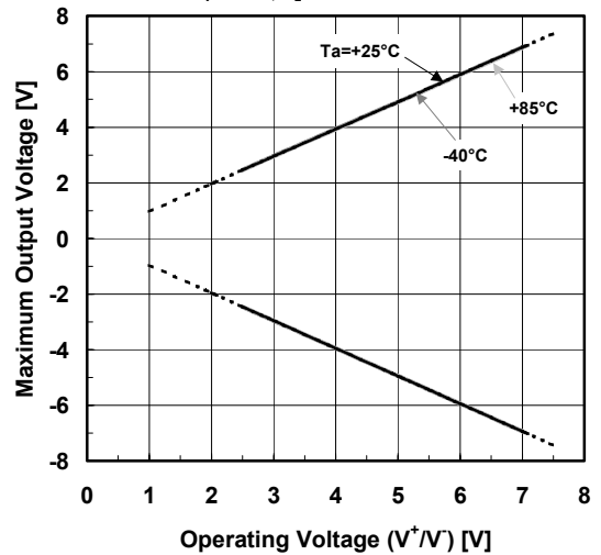
Maximum Output Voltage vs. Operating Voltage G_V = \text{OPEN} , R_L = 10\text{k}\Omega to GND
