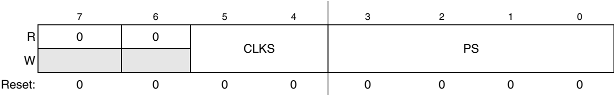
Figure 13-4. MTIM Clock Configuration Register (MTIMCLK)
