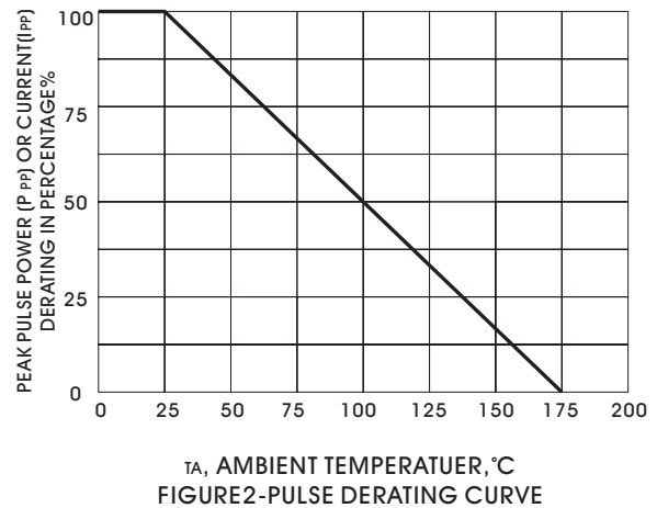
FIGURE 2-PULSE DERATING CURVE
