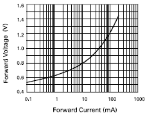
Forward Characteristics
