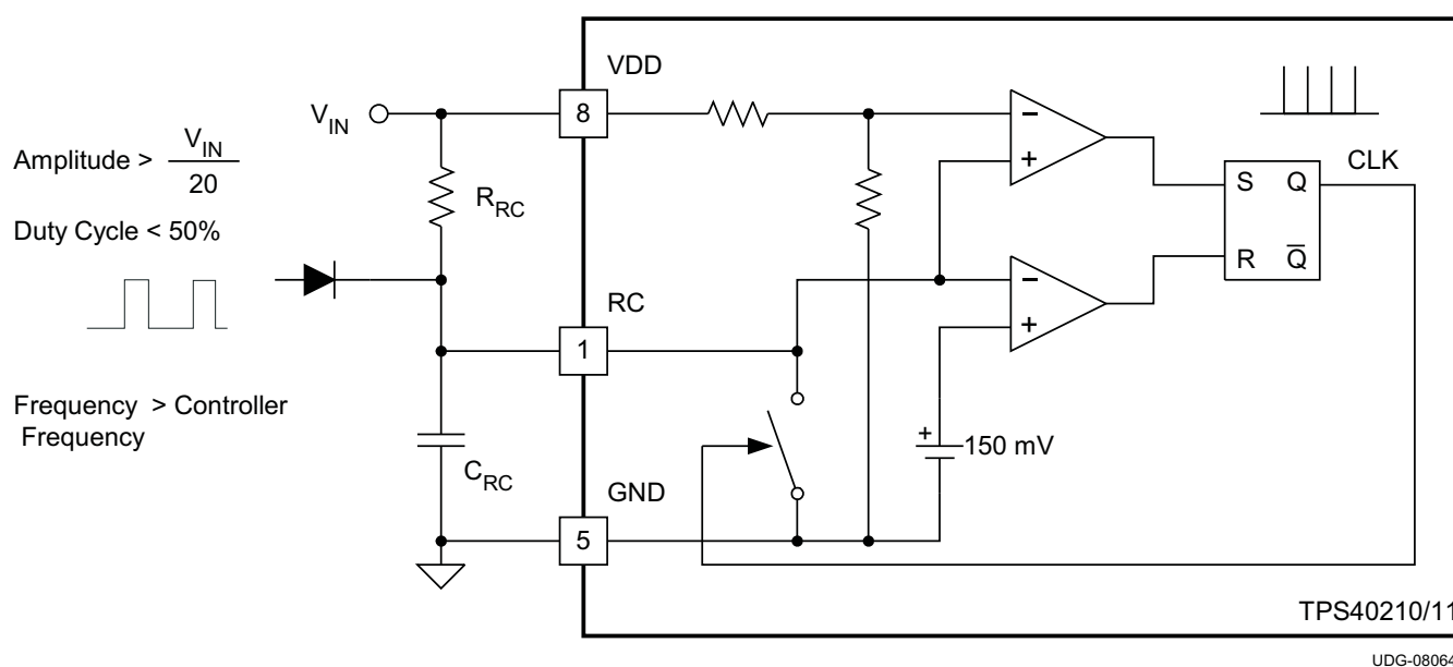
Figure 24. Diode Connected Synchronization
