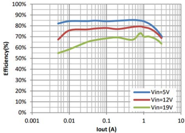
Fig3. Efficiency (Vout=5.0V)
