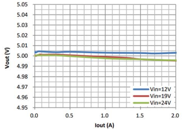
Fig6. Load Regulation (Vout=5.0V)
