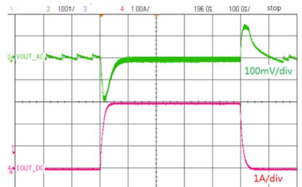
Fig10. Vin=12V, Vout=3.3V, C4=330pF, Iout= 0.01~3A Ch2—Vout, Ch4—I L
