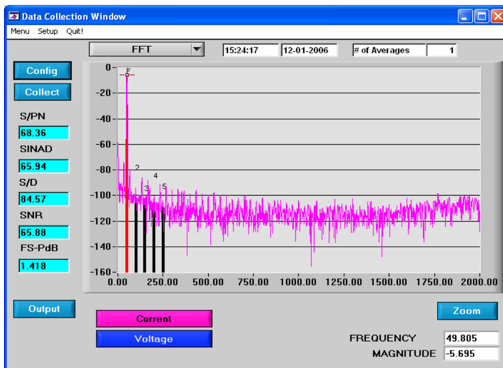
Figure 14. FFT Analysis
