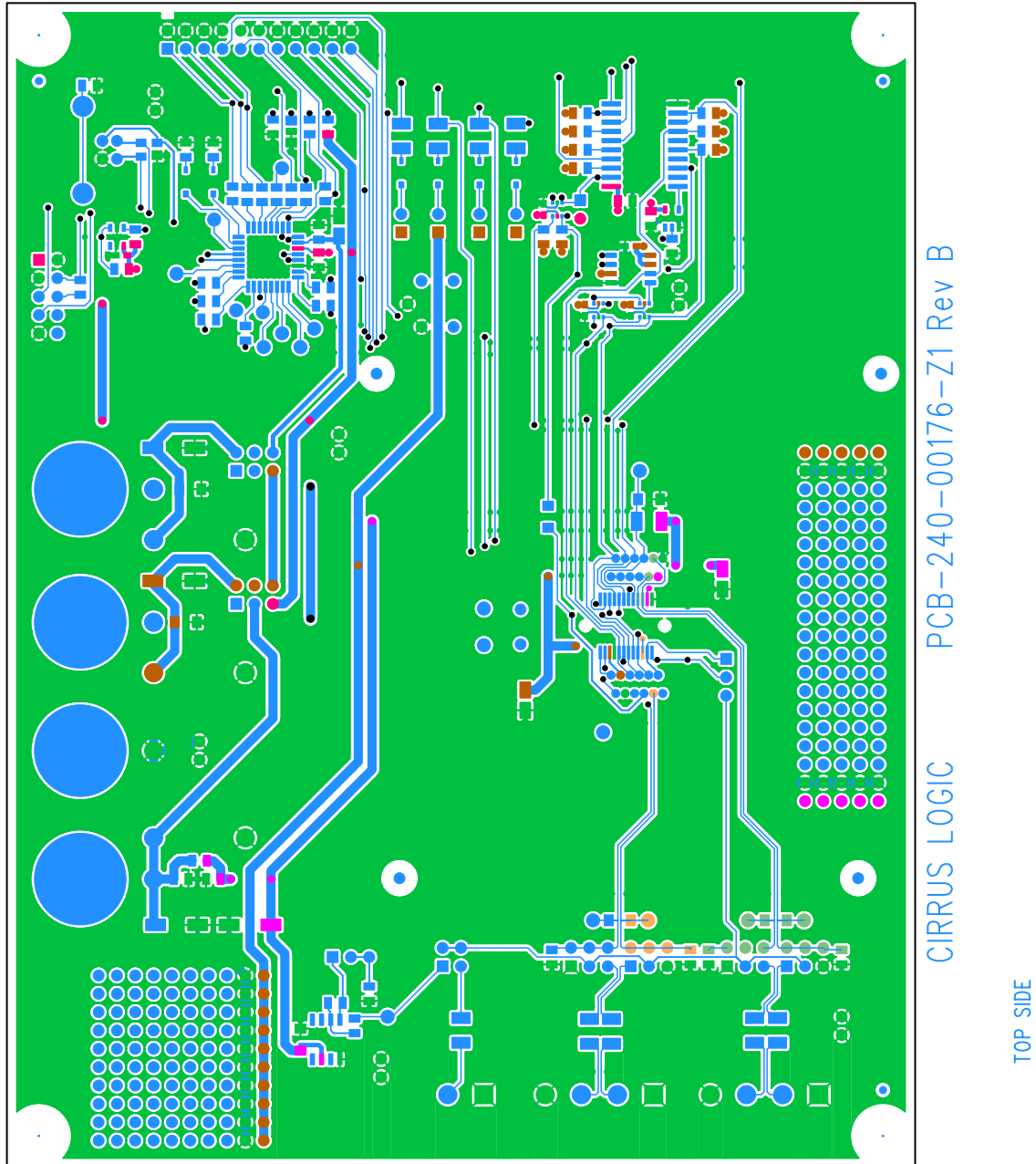
Figure 23. Topside Layer
