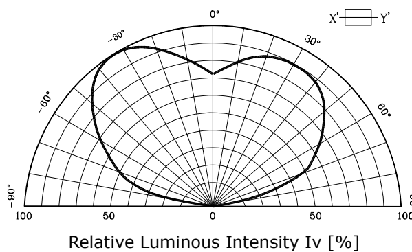
Fig. 5-2 Radiation Diagram(Y)
