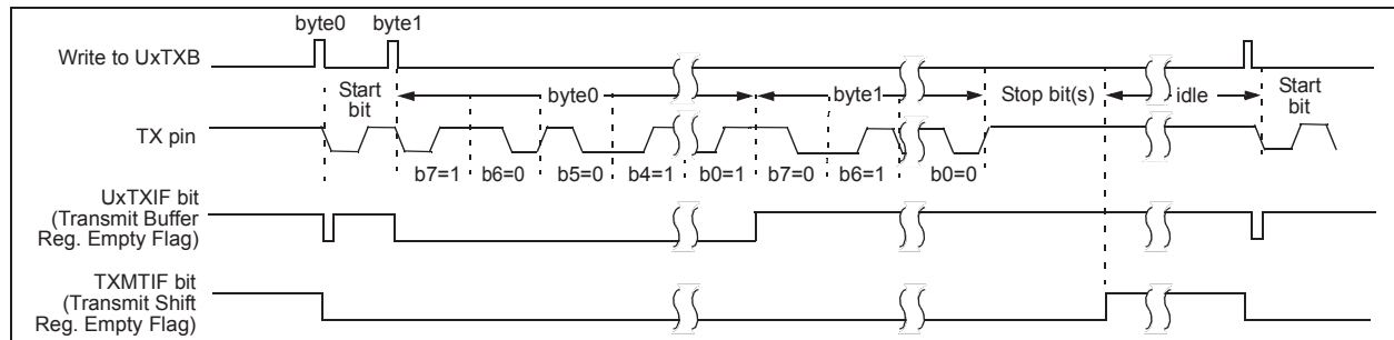
FIGURE 33-7: MANCHESTER TIMING
