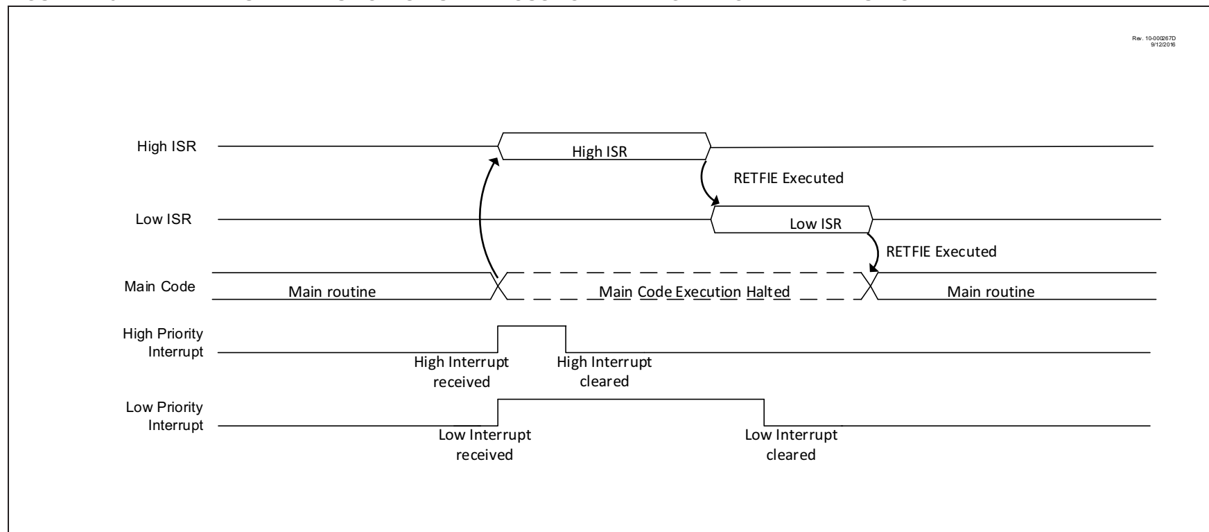
FIGURE 11-5: INTERRUPT EXECUTION: SIMULTANEOUS LOW AND HIGH PRIORITY INTERRUPTS
