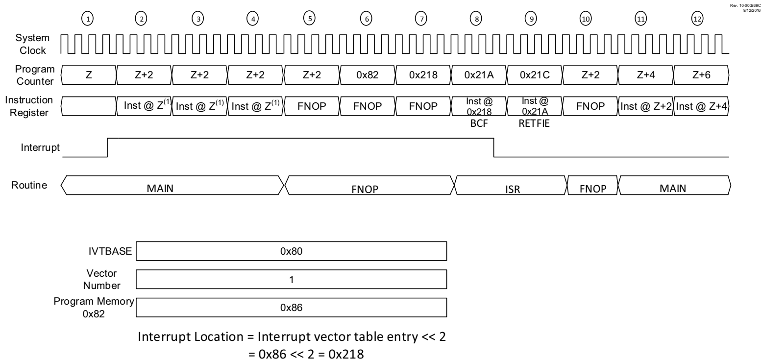
FIGURE 11-9: INTERRUPT TIMING DIAGRAM - THREE CYCLE INSTRUCTION
