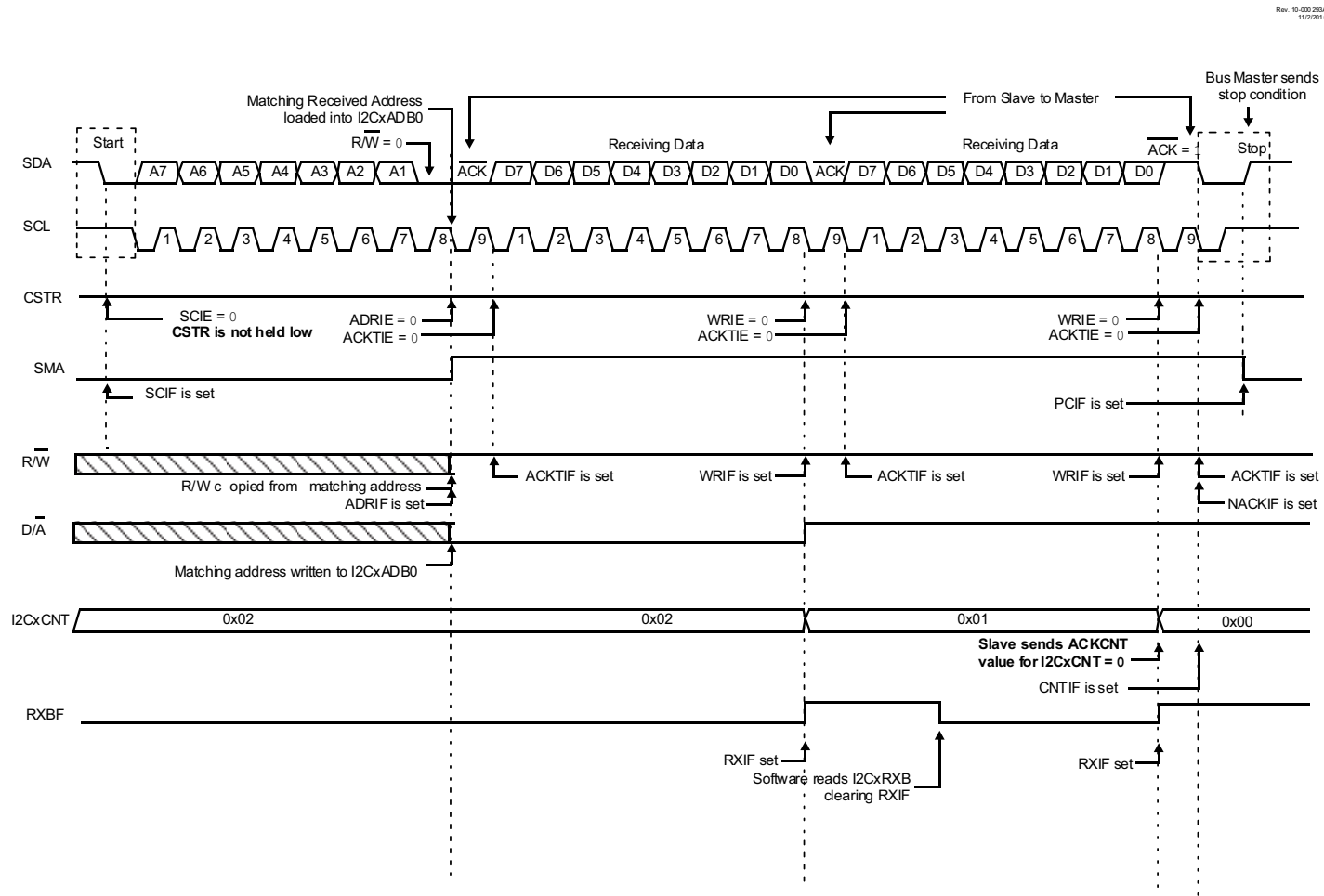
FIGURE 35-6: I 2 C SLAVE, 7-BIT ADDRESS, RECEPTION (ACKTIE = 0, ADRIE = 0, WRIE = 0)
