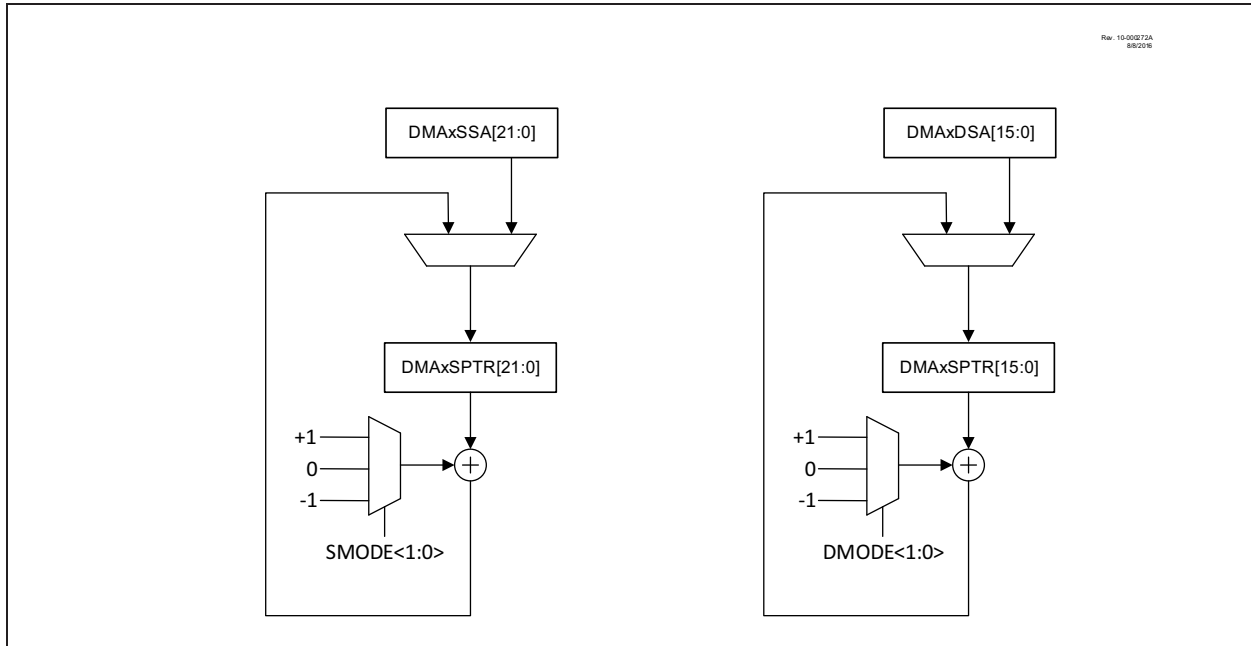
FIGURE 17-2: DMA POINTERS BLOCK DIAGRAM
