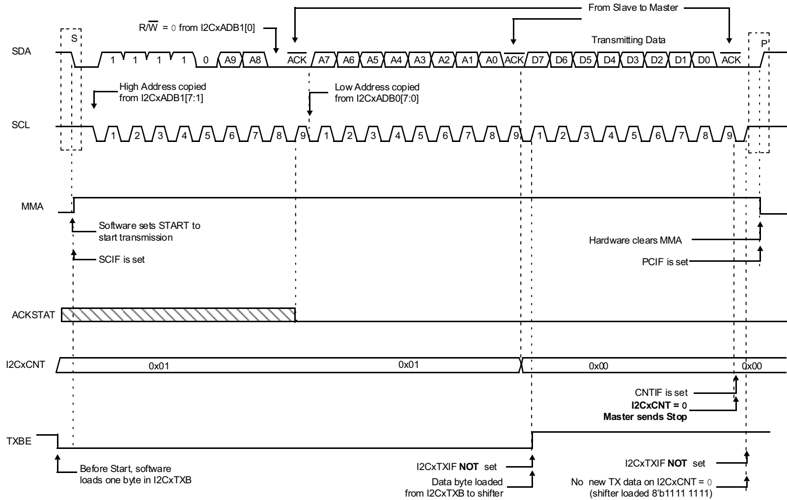
FIGURE 35-21: I 2 C MASTER, 10-BIT ADDRESS, TRANSMISSION WITH STOP
