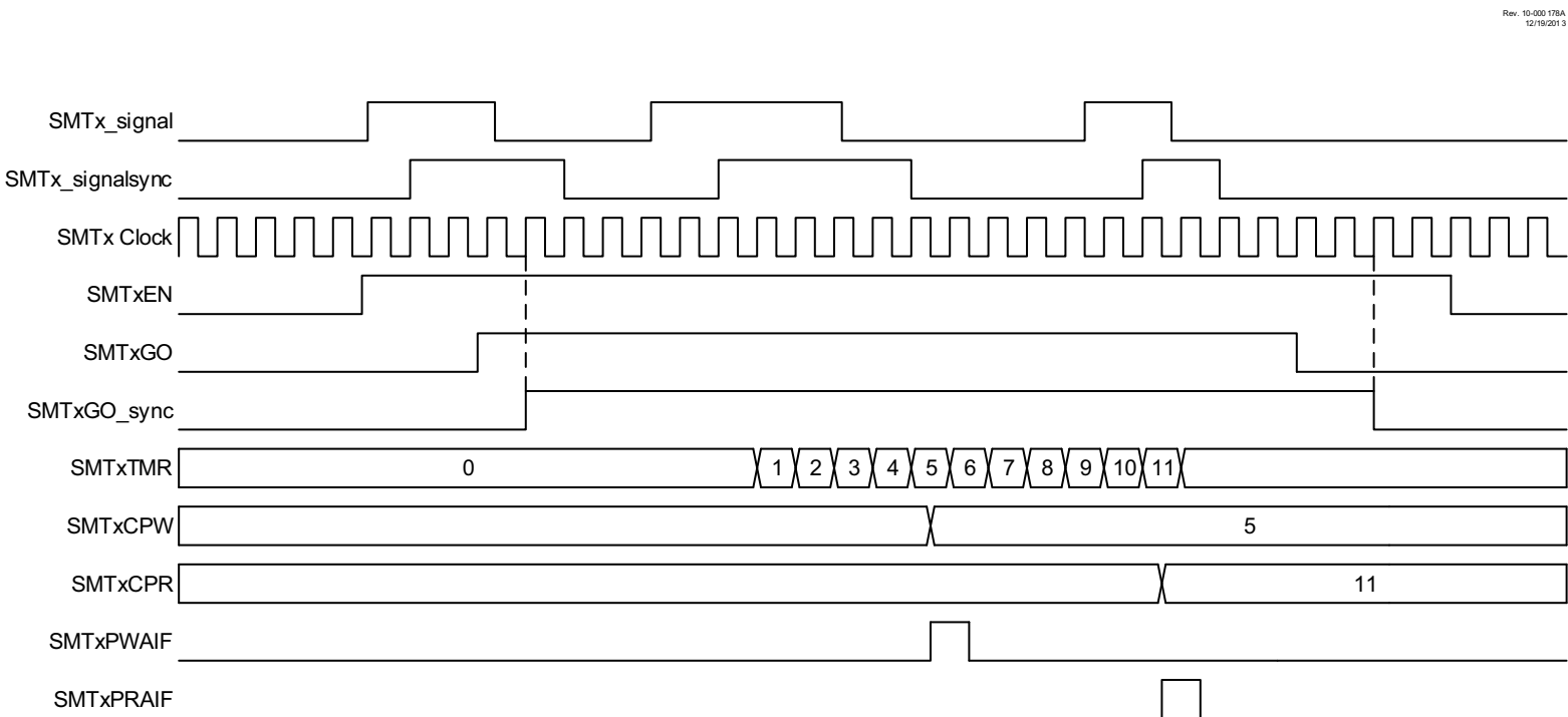
FIGURE 27-7: PERIOD AND DUTY-CYCLE SINGLE ACQUISITION TIMING DIAGRAM
