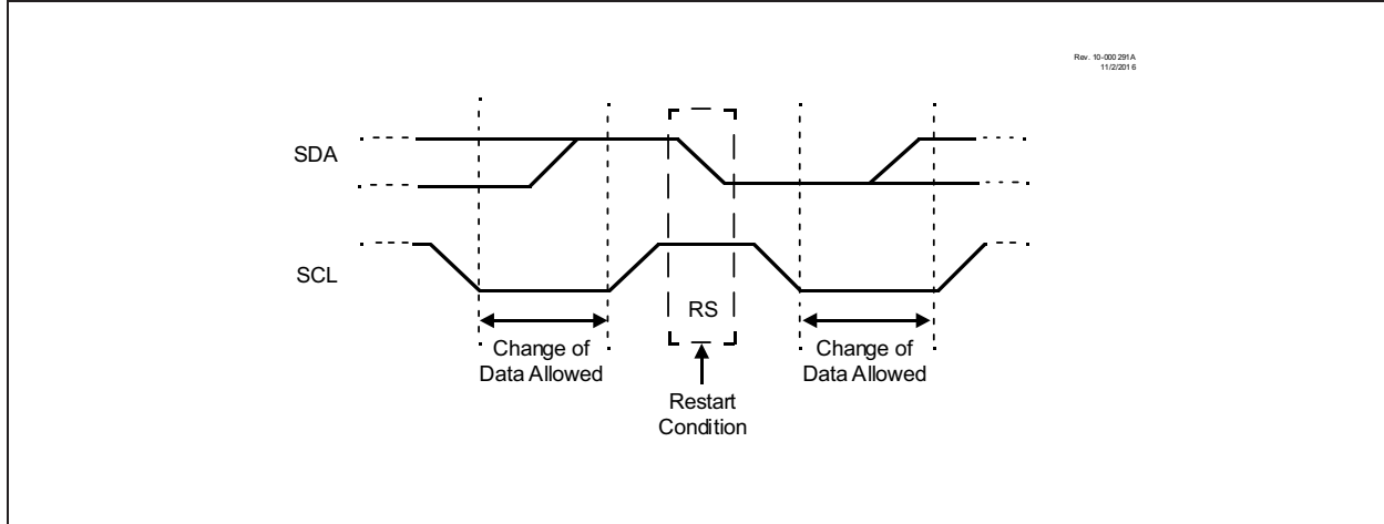
FIGURE 35-4: RESTART CONDITION
