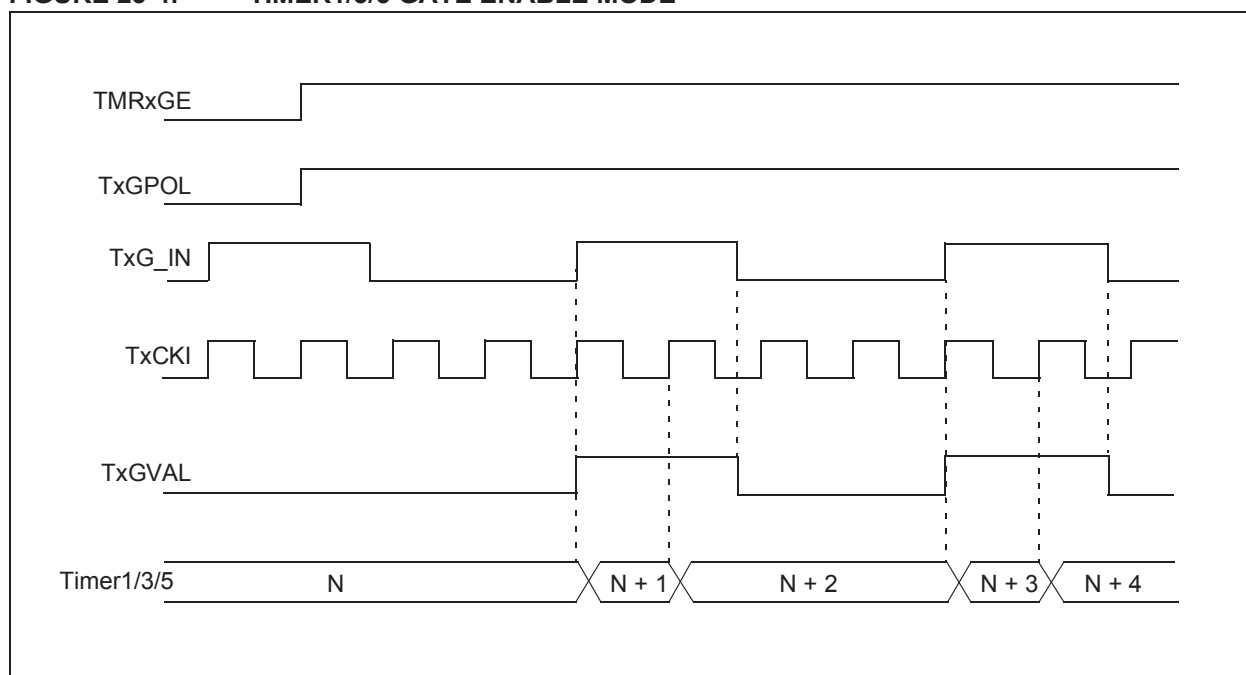
FIGURE 23-4: TIMER1/3/5 GATE ENABLE MODE
