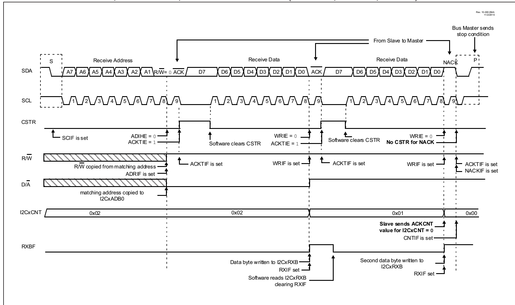
FIGURE 35-7: I 2 C SLAVE, 7-BIT ADDRESS, RECEPTION WITH I2CxCNT (ACKTIE = 1, ADRIE = 0, WRIE = 0)
