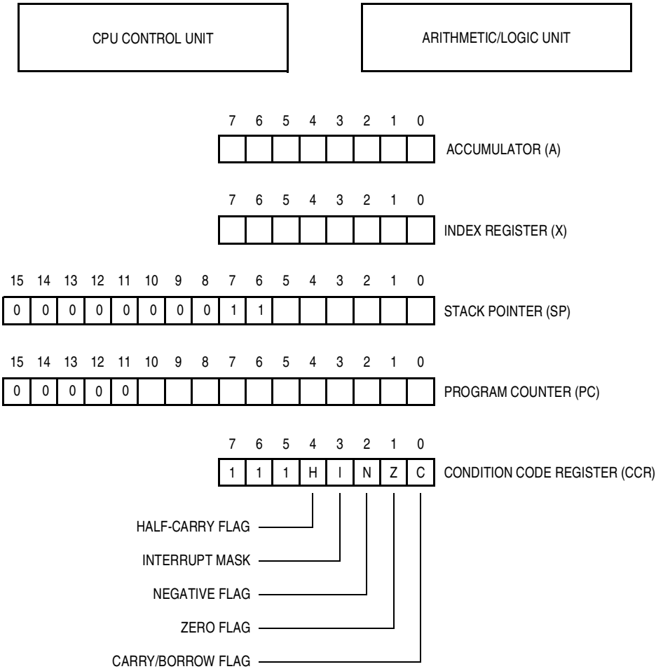
Figure 3-1. Programming Model
