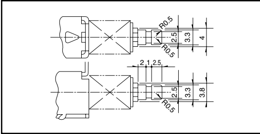
■ Actuator Configuration at Front Edge Unit:mm
