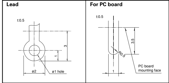
■ Terminal Configuration
