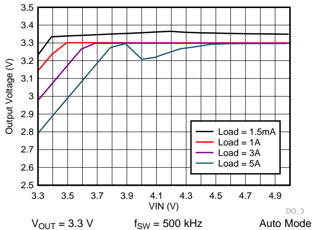
Figure 55. LM73605 Dropout Curve
