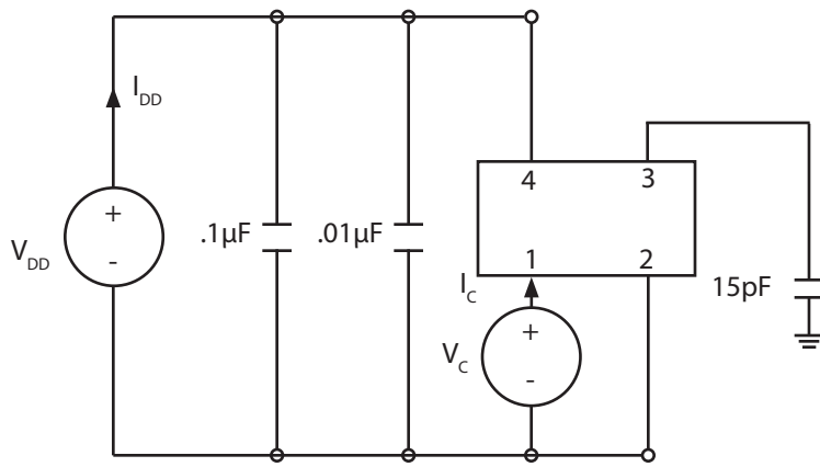
Fig 1: Test Circuit
