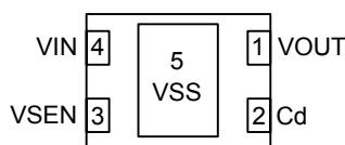
USP-4 (BOTTOM VIEW)
