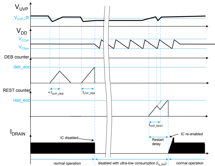
Figure 29. UVP timing
