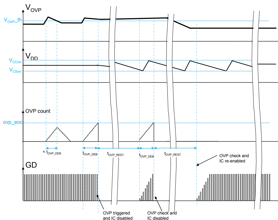
Figure 32. OVP timing
