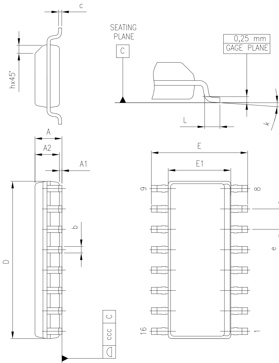
Figure 46. SO16N package outline
