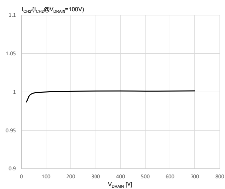
Figure 12. I_{CH2} vs. V_{DRAIN}
