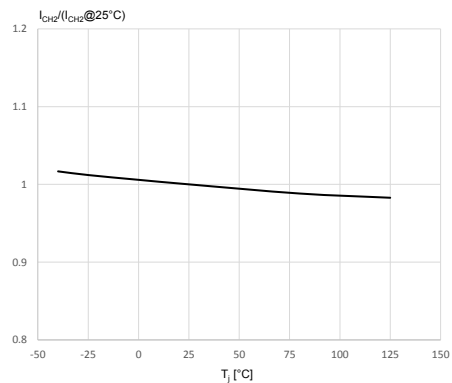
Figure 10. I_{CH2} vs. T_J
