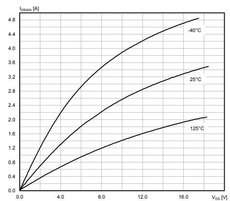
Figure 20. Output characteristic
