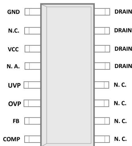
Figure 1. Connection diagram
