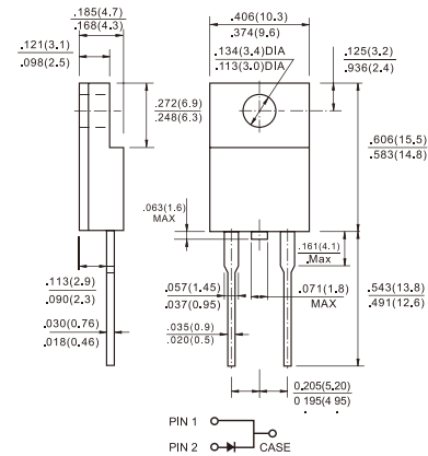
Dimensions in inches and (millimeters) Marking Diagram
