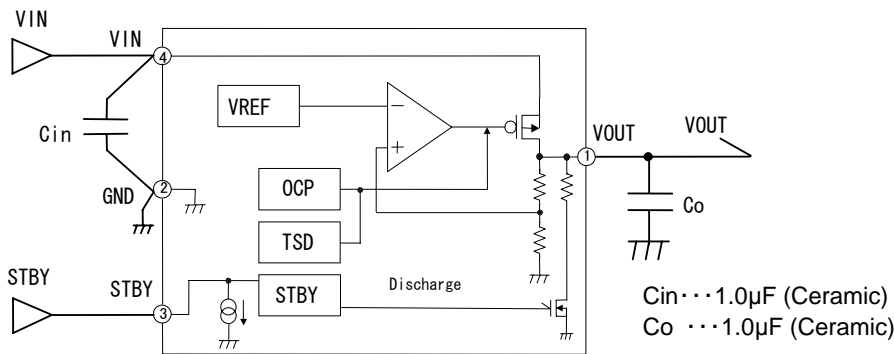
Fig. 2 Block Diagrams
