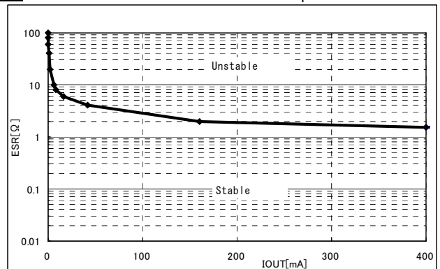
Fig. 24 Stable region (example)
