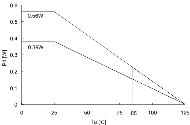
Fig. 23 SSON04X1010 Power dissipation heat reduction characteristics (Reference)
