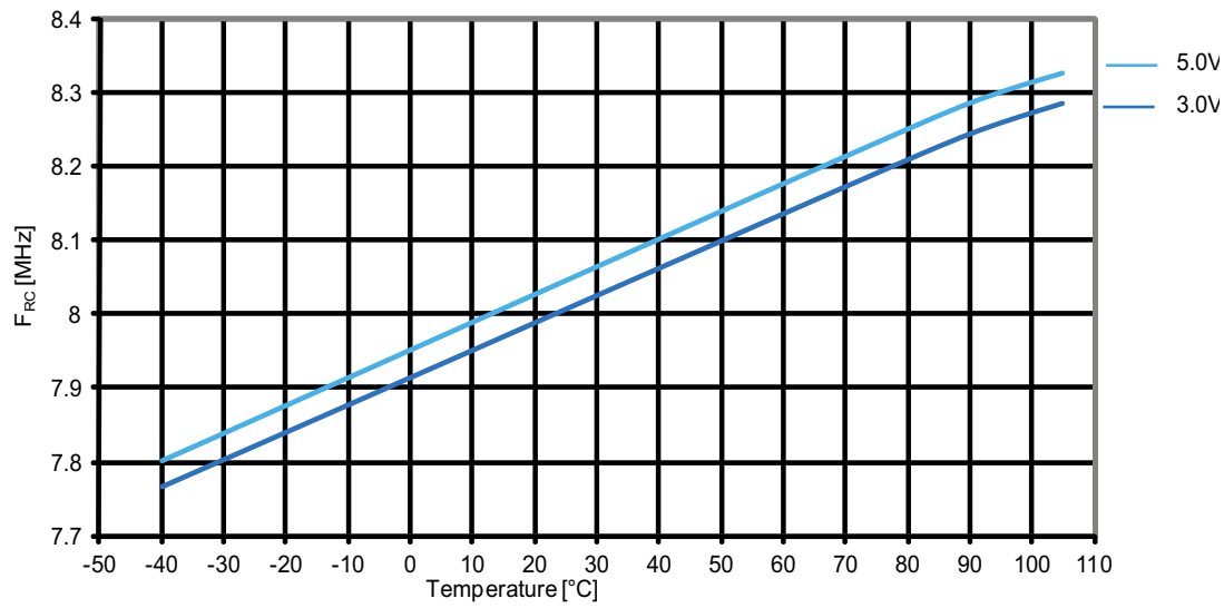
Figure 31-33. ATmega164PA: Calibrated 8MHz RC oscillator vs. temperature
