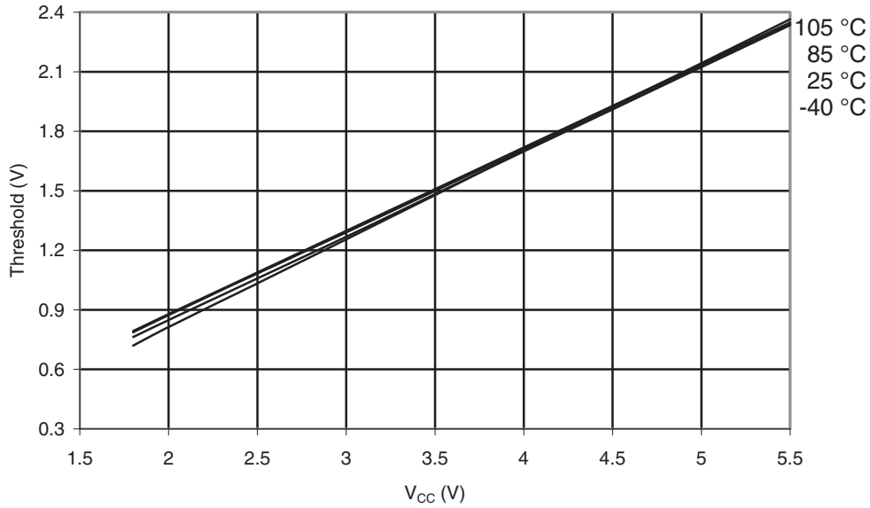
Figure 31-103. Reset Pin Input Threshold vs. V_{CC} ( V_{IL} , I/O Pin Read as '0')
