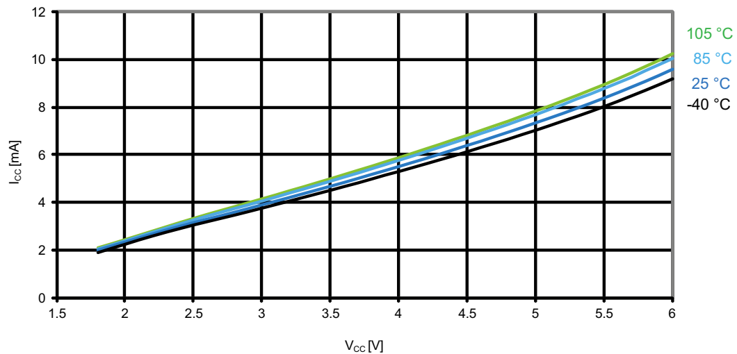
Figure 31-120. ATmega1284P: Active supply current vs. V_{CC} (internal RC oscillator, 8MHz)
