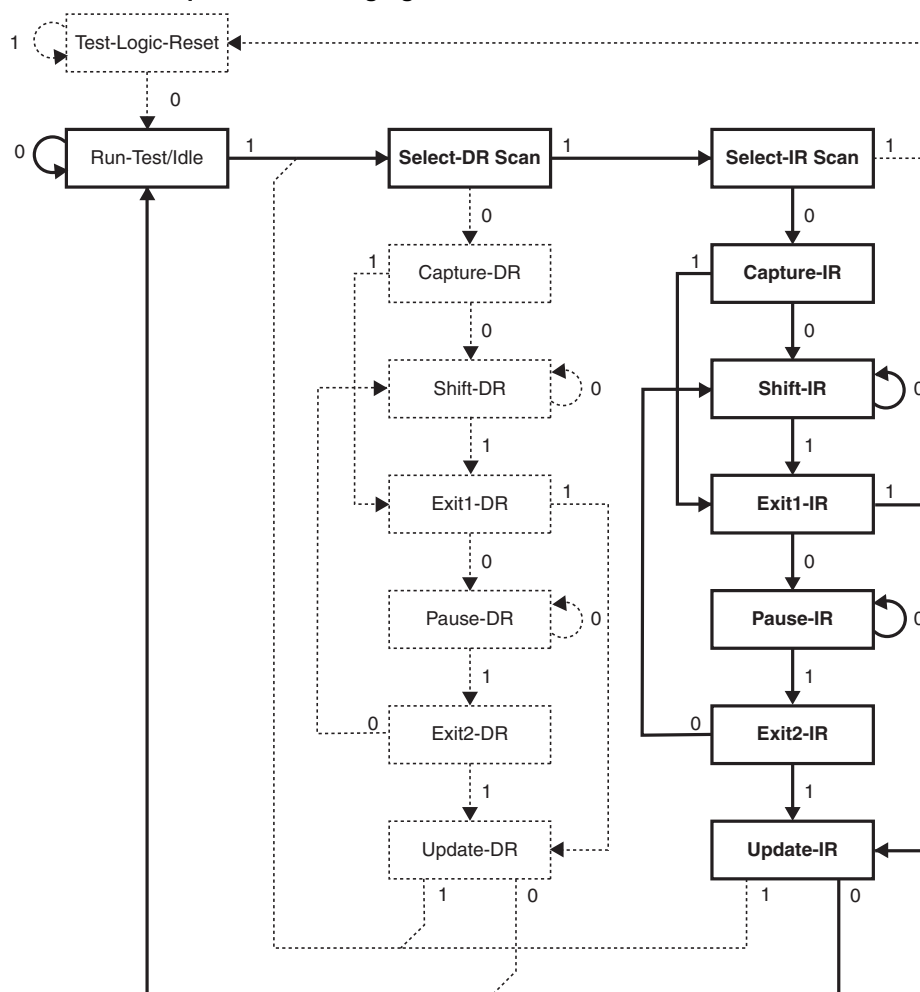
Figure 27-13. State machine sequence for changing the instruction word
