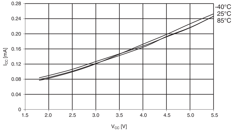
Figure 30-299. ATmega1284: Active supply current vs. V_{CC} (internal RC oscillator, 128kHz)
