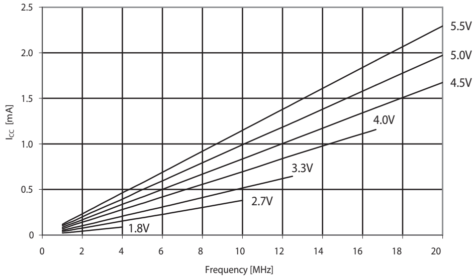
Figure 30-195. ATmega324PA: Reset supply current vs. frequency (1 - 20MHz)
