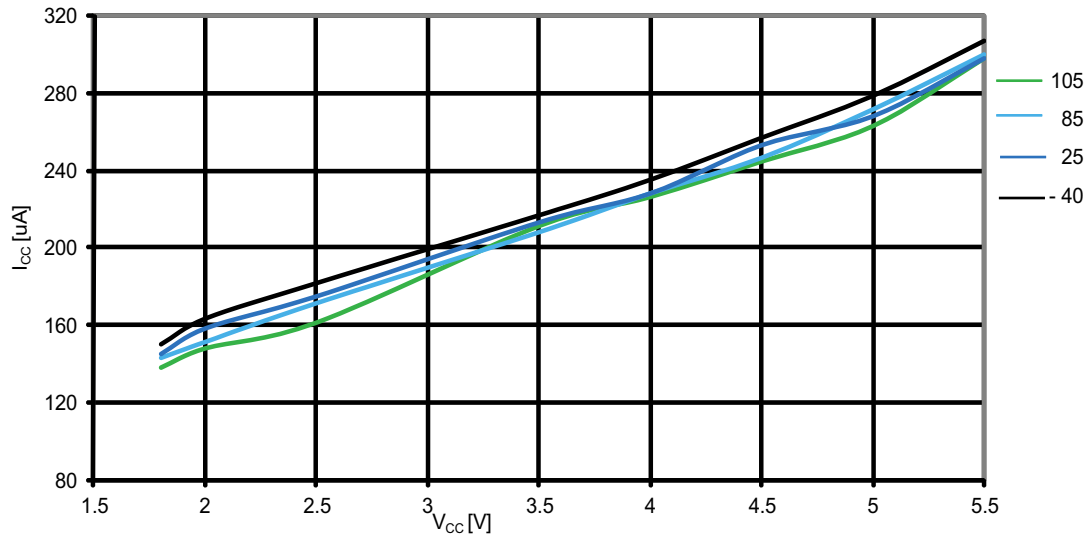
Figure 31-35. ATmega164PA: ADC current vs. V_{CC} (AREF = AV_{CC} )
