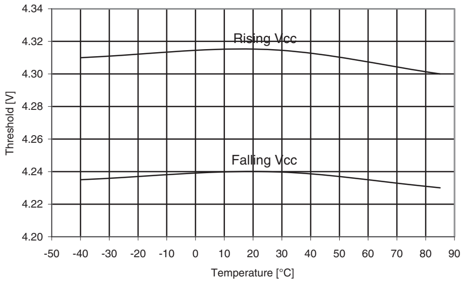
Figure 30-80. ATmega164PA: BOD threshold vs. temperature ( V_{BOT} = 4.3V )
