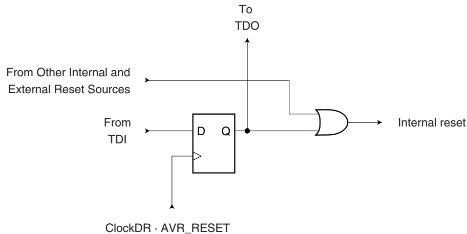
Figure 25-2. Reset register
