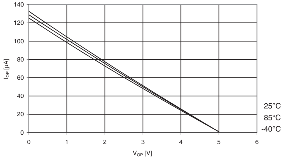
Figure 30-17. ATmega164A: I/O pin pull-up resistor current vs. input voltage ( V_{CC} = 5V )
