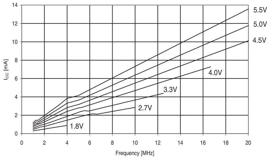
Figure 30-247. ATmega644PA: Active supply current vs. frequency (1 - 20MHz)
