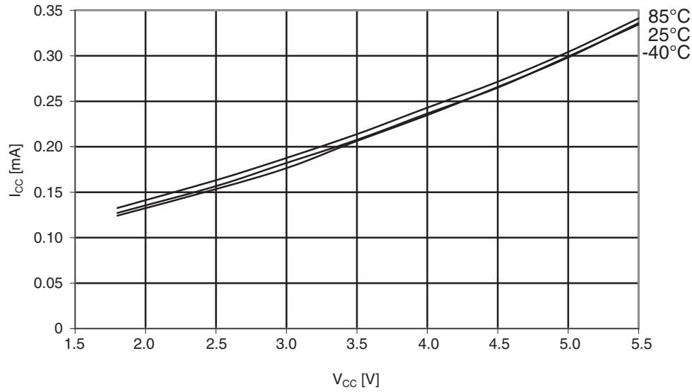
Figure 30-205. ATmega644A: Idle supply current vs. V_{CC} (internal RC oscillator, 1MHz)
