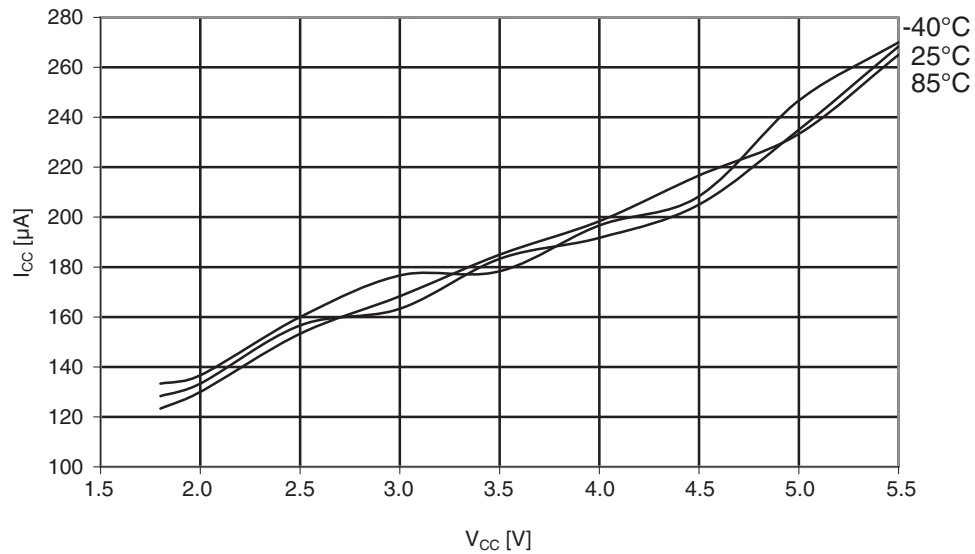
Figure 30-386. ATmega1284P: ADC current vs. V_{CC} (AREF = AV_{CC} )
