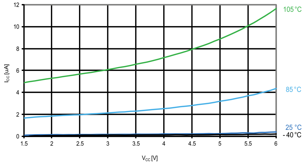
Figure 31-126. ATmega1284P: Power-down supply current vs. V_{CC} (watchdog timer disabled)
