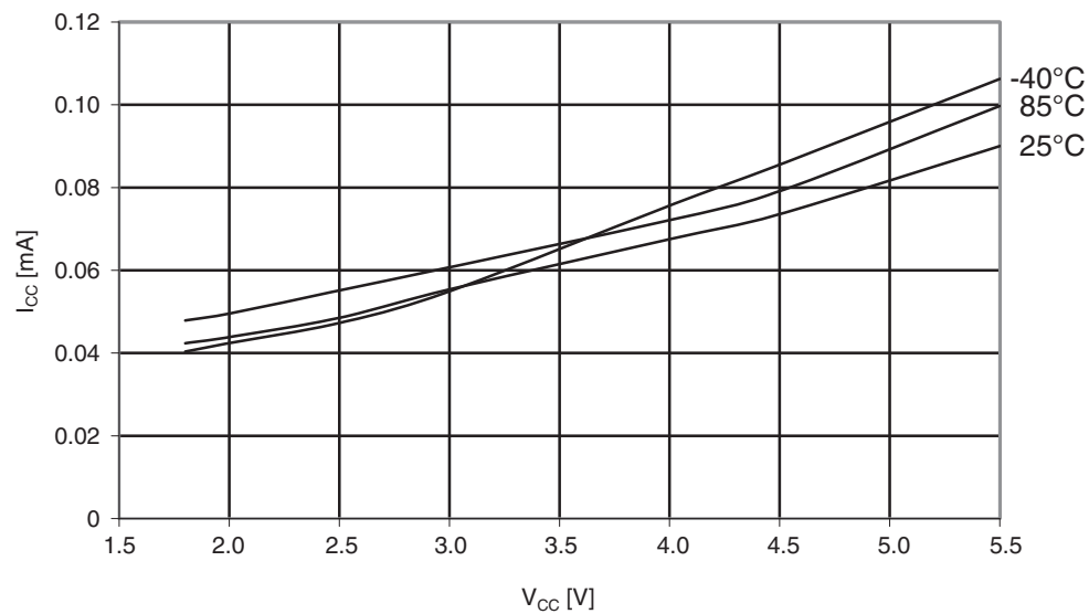
Figure 30-304. ATmega1284: Idle supply current vs. V_{CC} (internal RC oscillator, 128kHz)
