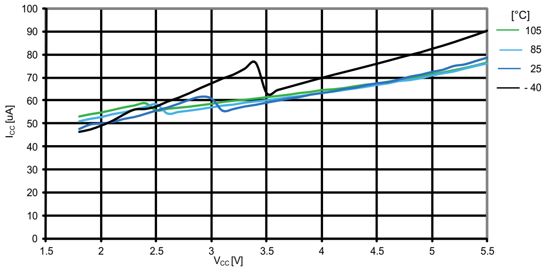
Figure 31-36. ATmega164PA: Analog comparator current vs. V_{CC}
