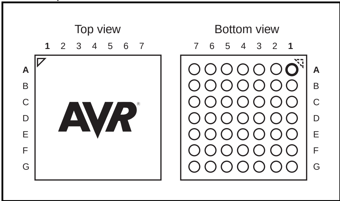
Figure 1-3. VFBGA - pinout
