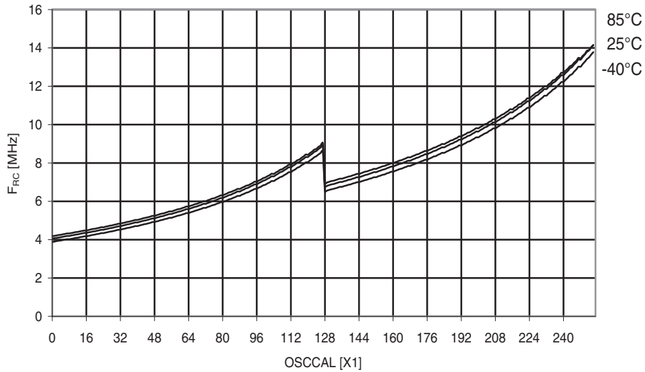
Figure 30-236. ATmega644A: Calibrated 8MHz RC oscillator vs. OSCAL value
