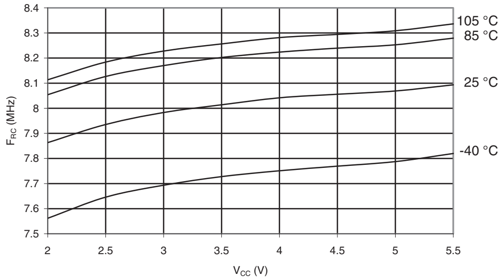
Figure 31-110. Calibrated 8 MHz RC Oscillator vs. V_{CC}
