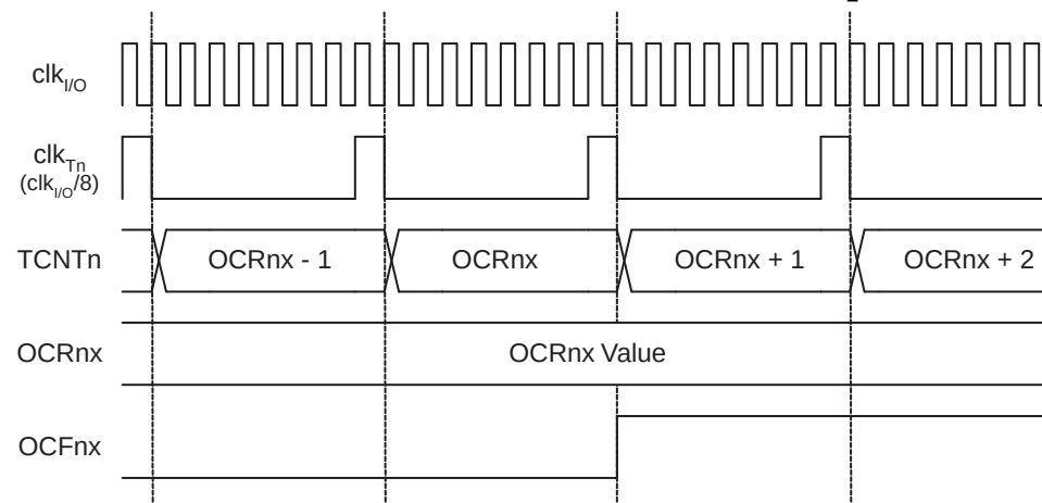
Figure 16-11. Timer/Counter Timing diagram, setting of OCFnx, with prescaler ( f_{\text{clk}_{\text{I/O}}}/8 )
