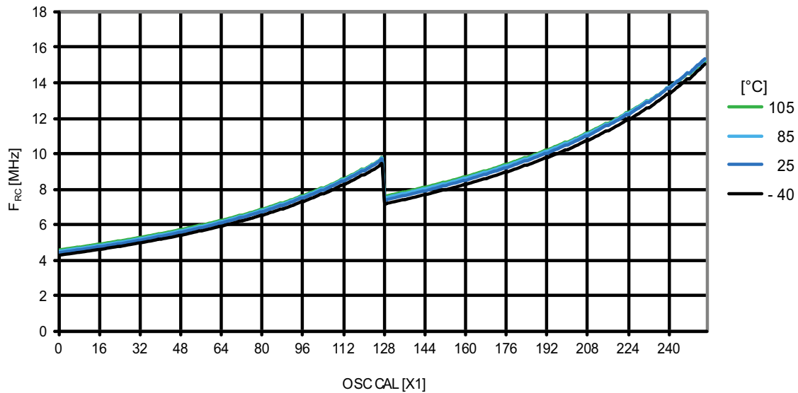
Figure 31-34. ATmega164PA: Calibrated 8MHz RC oscillator vs. OSCAL value
