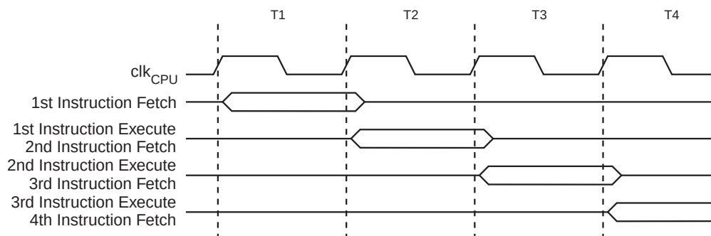
Figure 7-5. The Parallel Instruction Fetches and Instruction Executions
