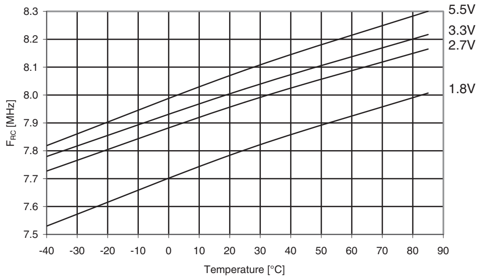
Figure 30-334. ATmega1284: Calibrated 8MHz RC oscillator vs. temperature
