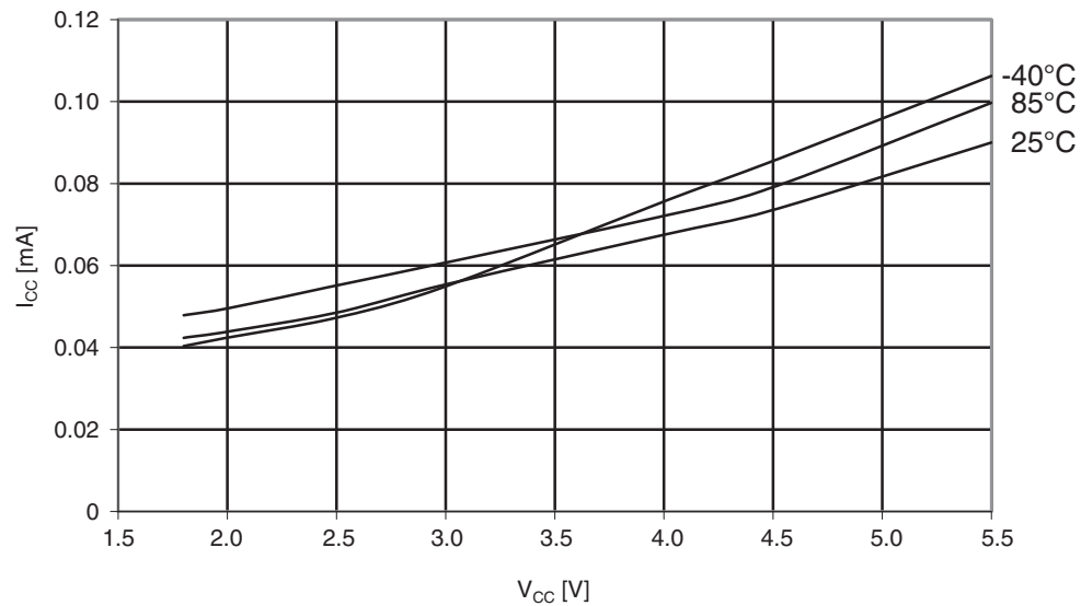
Figure 30-354. ATmega1284P: Idle supply current vs. V_{CC} (internal RC oscillator, 128kHz)
