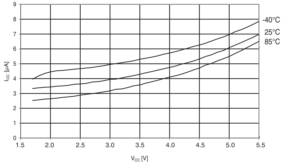
Figure 30-242. ATmega644A: Watchdog timer current vs. V_{CC}
