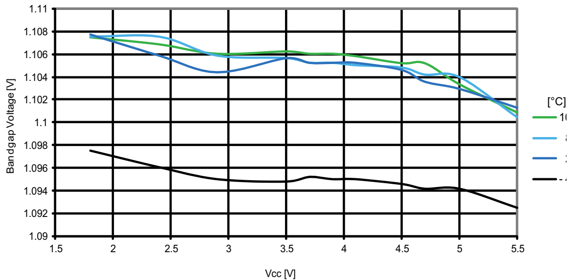
Figure 31-28. ATmega164PA: Calibrated bandgap voltage vs. V_{CC}
