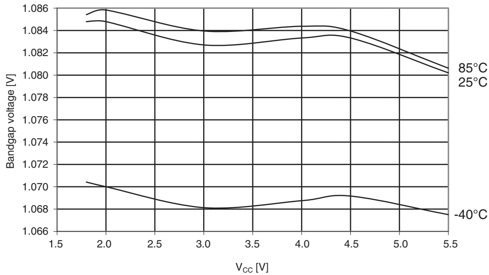
Figure 30-230. ATmega644A: Calibrated bandgap voltage vs. V_{CC}
