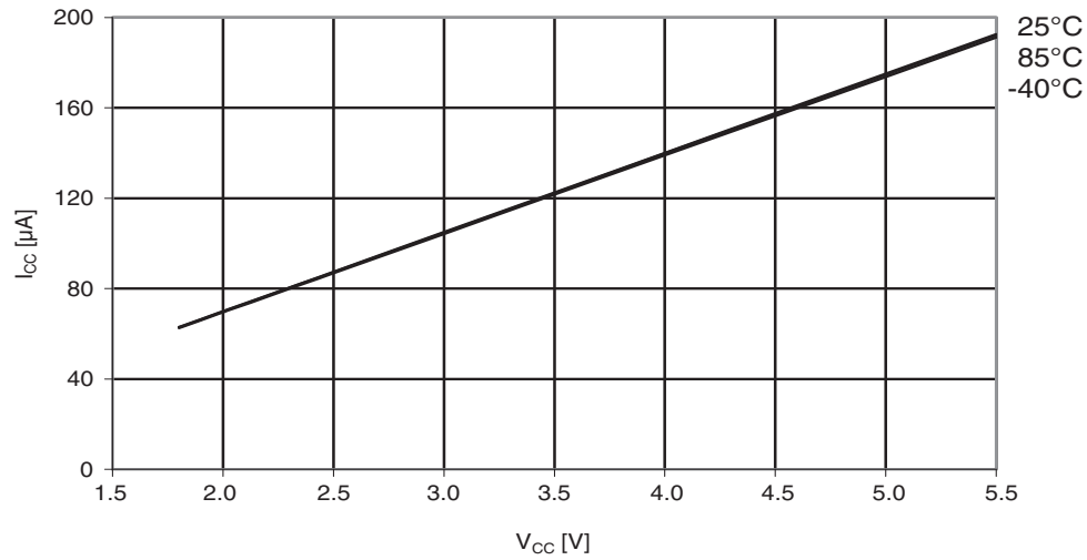
Figure 30-92. ATmega164PA: AREF external reference current vs. V_{CC}
