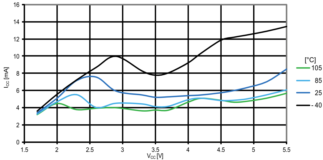
Figure 31-160. ATmega1284P: Programming current vs. V_{CC}
