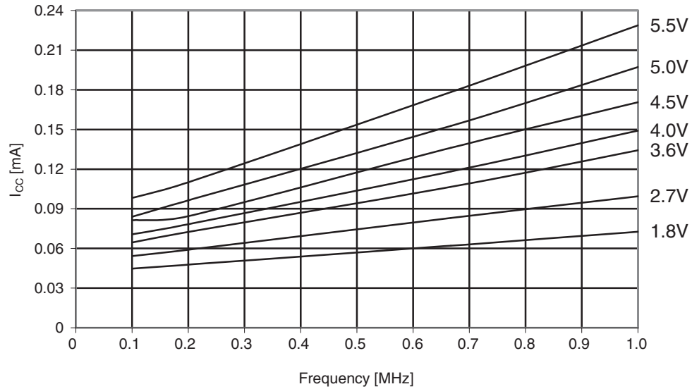
Figure 30-350. ATmega1284P: Idle supply current vs. low frequency (0.1 - 1.0MHz)
