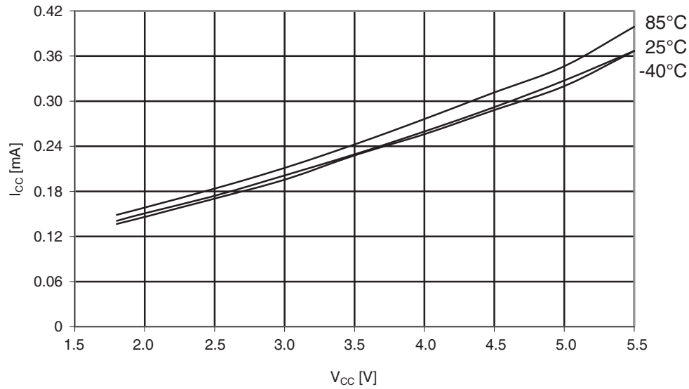
Figure 30-303. ATmega1284: Idle supply current vs. V_{CC} (internal RC oscillator, 1MHz)
