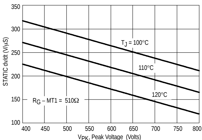
Figure 12.0 Typical Exponential Static dv/dt Versus Peak Voltage, MT2(-)
