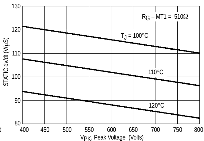
Figure 10.0 Typical Exponential Static dv/dt Versus Peak Voltage, MT2(+)
