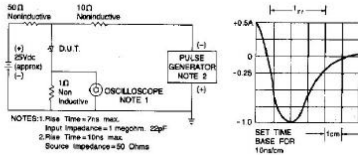
Fig. 6-REVERSE RECOVERY TIME CHARACTERISTIC AND TEST CIRCUIT DIAGRAM
