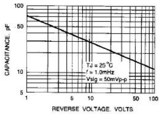
Fig. 5-TYPICAL JUNCTION CHARACTERISTICS
