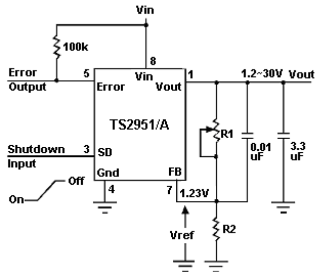
Figure 2. Adjust Voltage
