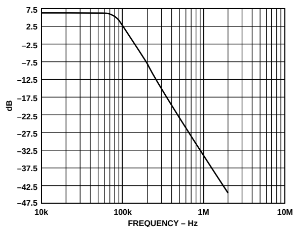
Figure 39. Frequency Response of Sallen-Key Filter
