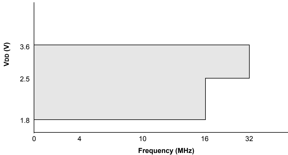
FIGURE 37-2: VOLTAGE FREQUENCY GRAPH, -40^{\circ}\text{C} \leq T_A \leq +125^{\circ}\text{C} , PIC16LF15356/75/76/85/86 ONLY
