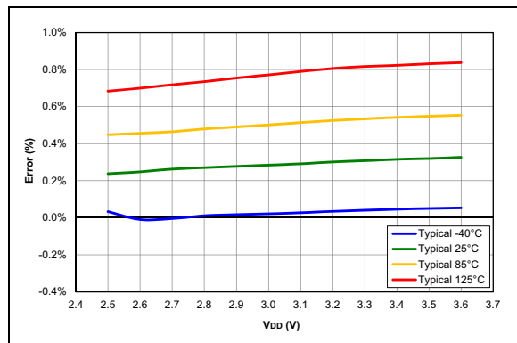
FIGURE 38-51: FVR Voltage Error 2X, PIC16LF15356/75/76/85/86 devices only
