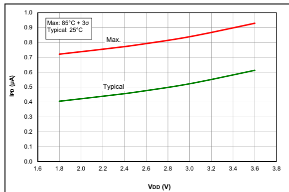
FIGURE 38-75: IPD, Watchdog Timer (WDT), PIC16LF15356/75/76/85/86 devices only
