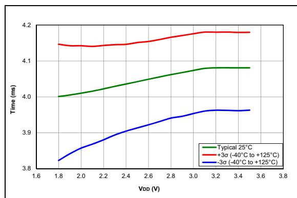
FIGURE 38-109: Watchdog Timer Time-out Period, PIC16LF15356/75/76/85/86 devices only
