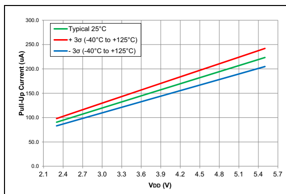
FIGURE 38-110: Weak Pull-up Current, PIC16F15356/75/76/85/86 devices only
