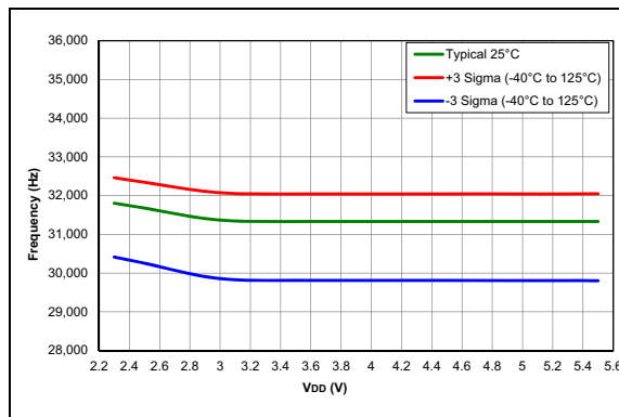
FIGURE 38-88: LFINTOSC Frequency, PIC16F15356/75/76/85/86 devices only
