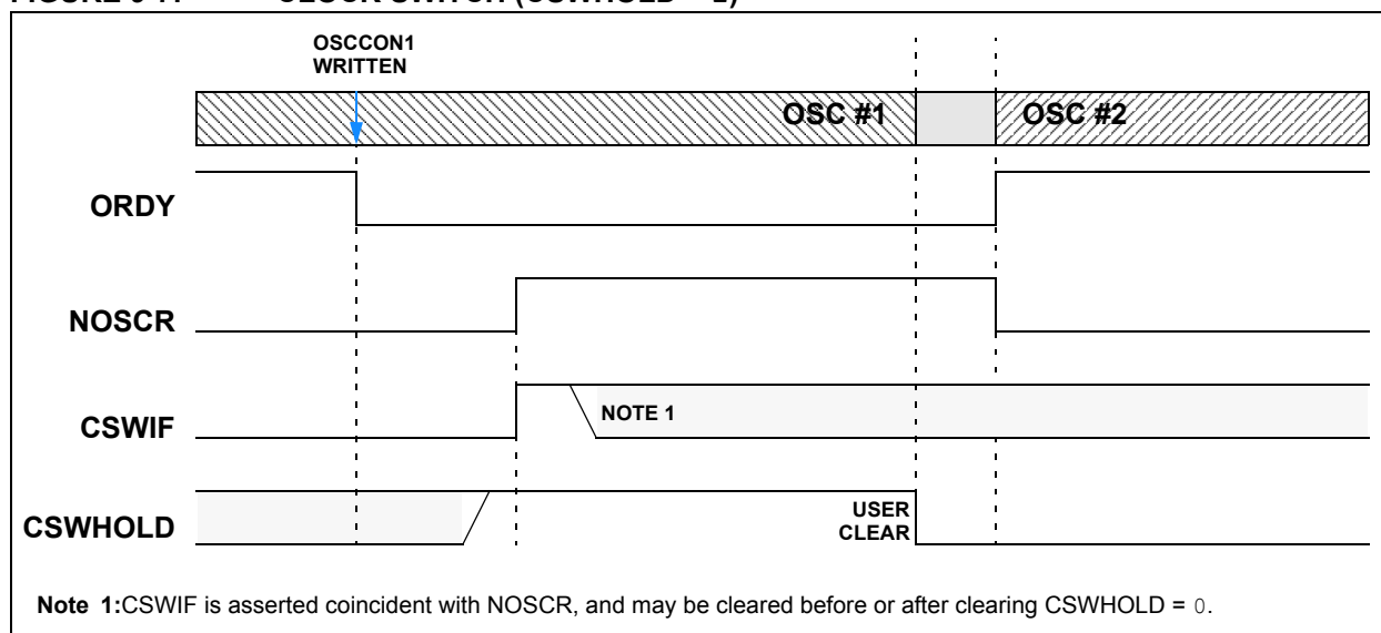
FIGURE 9-7: CLOCK SWITCH (CSWHOLD = 1)
