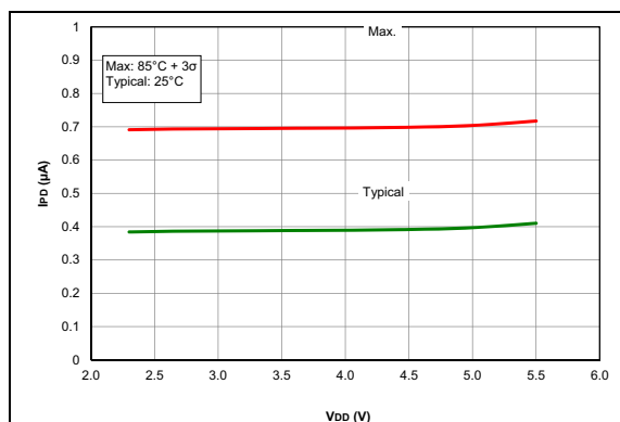
FIGURE 38-86: I_{pd} Base, 11, PIC16F15356/75/76/85/86 devices only
