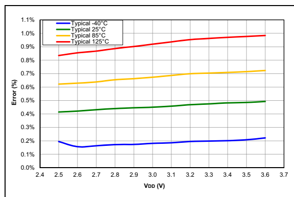
FIGURE 38-49: Typical FVR Voltage 1X, PIC16F15356/75/76/85/86 devices only
