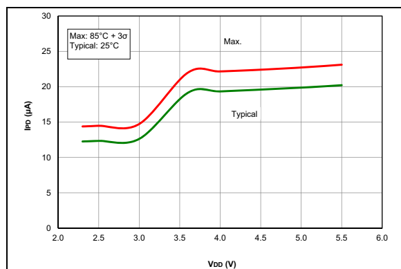
FIGURE 38-85: I_{pd} Base, 01, PIC16F15356/75/76/85/86 devices only
