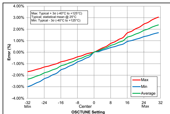
FIGURE 38-89: OCSTUNE Center Frequency, PIC16(L)F15356/75/76/85/86 devices only
