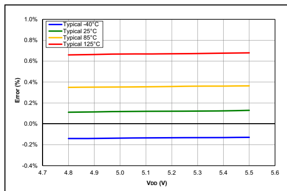
FIGURE 38-53: FVR Voltage Error 4X, PIC16F15356/75/76/85/86 devices only
