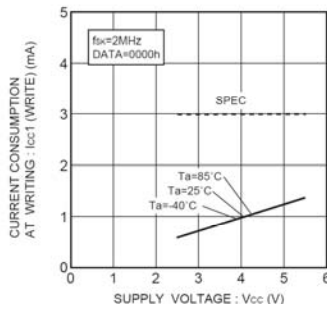
Fig.12 Current consumption at WRITE action ICC1(WRITE, f_{SK}=2MHz)
