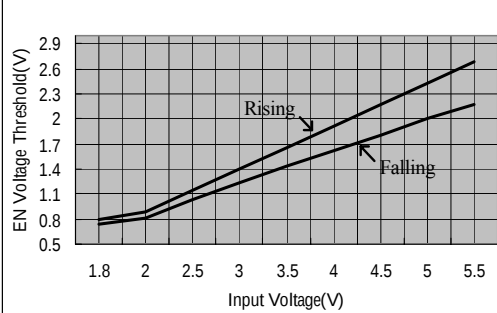
EN Voltage Threshold vs. Input Voltage
