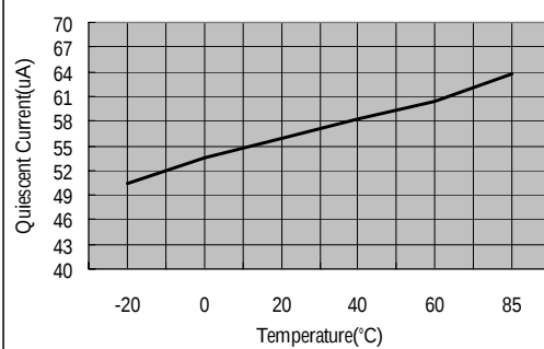
Quiescent Current vs. Temperature
