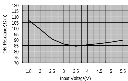
ON-Resistance vs. Input Voltage
