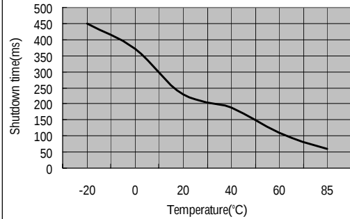
Short circuit Shutdown time vs. Temperature
