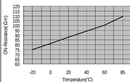
ON-Resistance vs. Temperature
