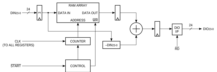
FIGURE 6. DELAY AND SUBTRACT MODE
