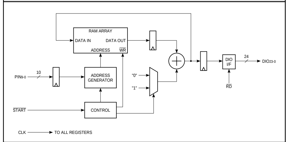
FIGURE 1. HISTOGRAM MODE
