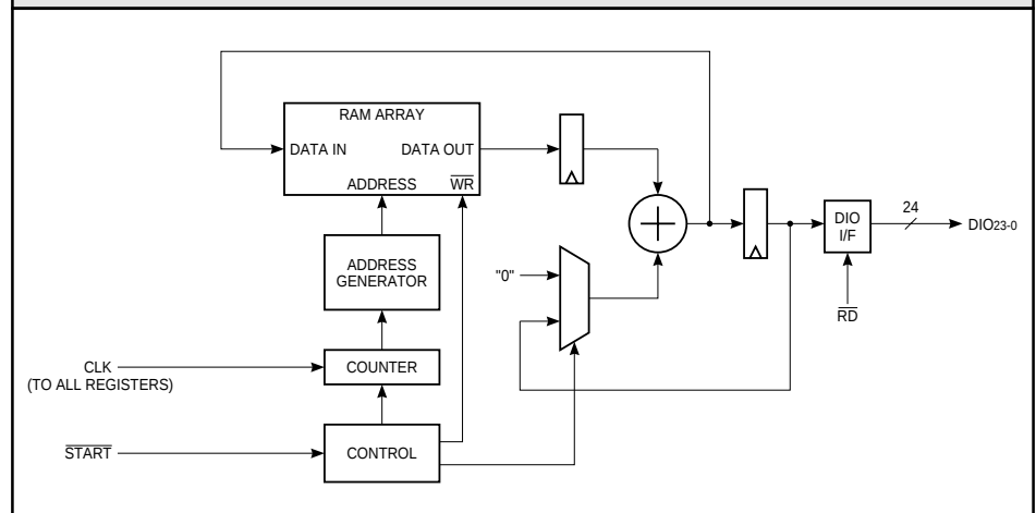
FIGURE 2. HISTOGRAM ACCUMULATE MODE
