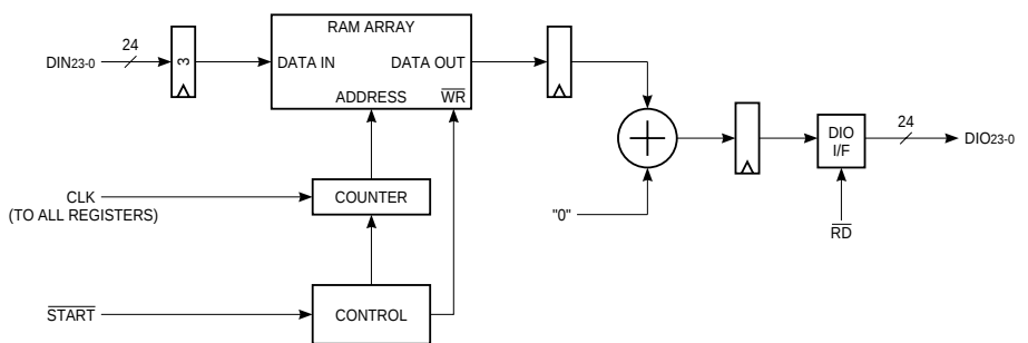
FIGURE 5. DELAY MEMORY MODE
