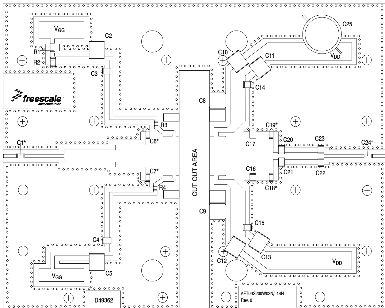
Figure 2. AFT09S200W02NR3 Test Circuit Component Layout — 920–960 MHz
